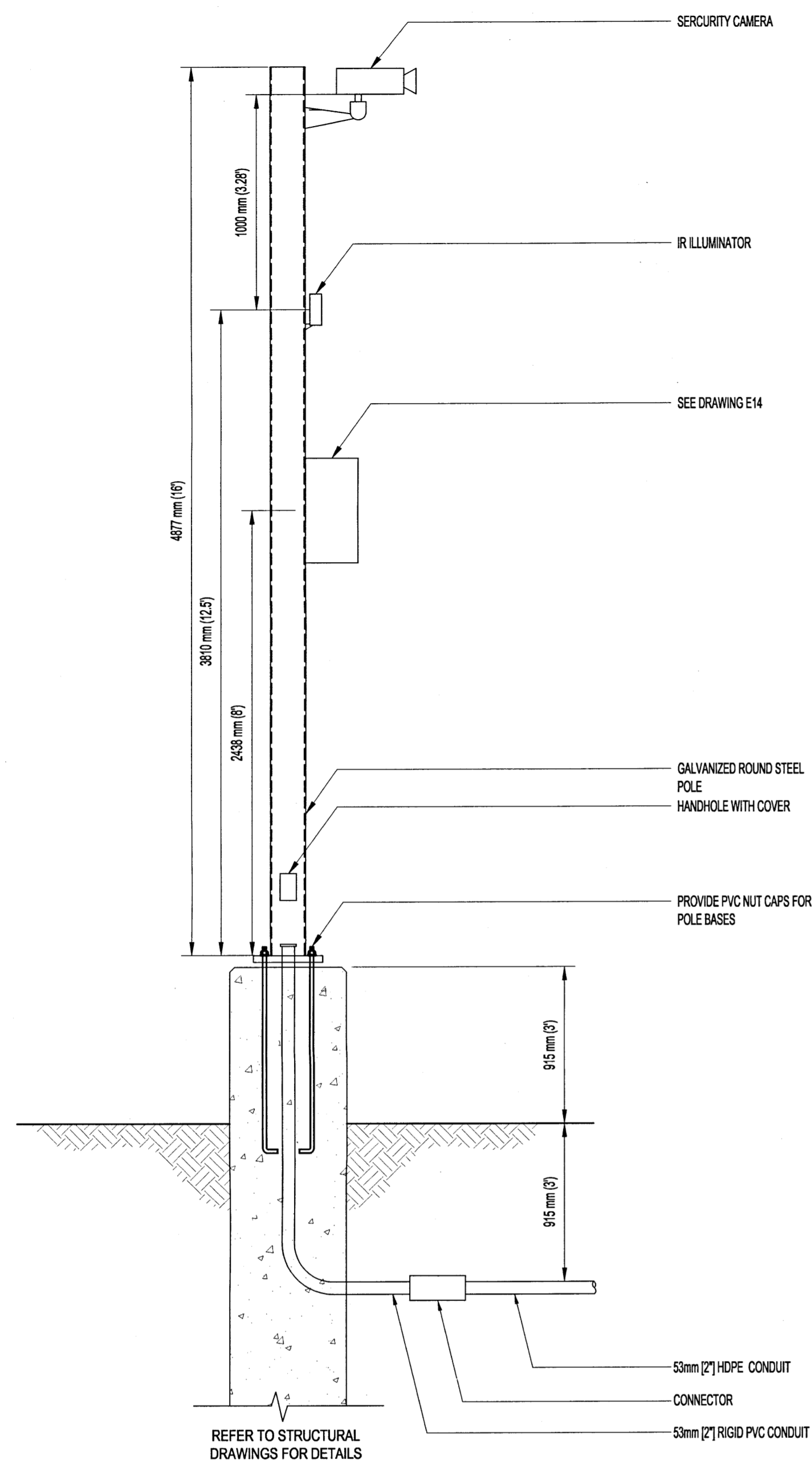
A TYPICAL SECURITY CAMERA POLE MOUNTING DETAIL N.T.S.
