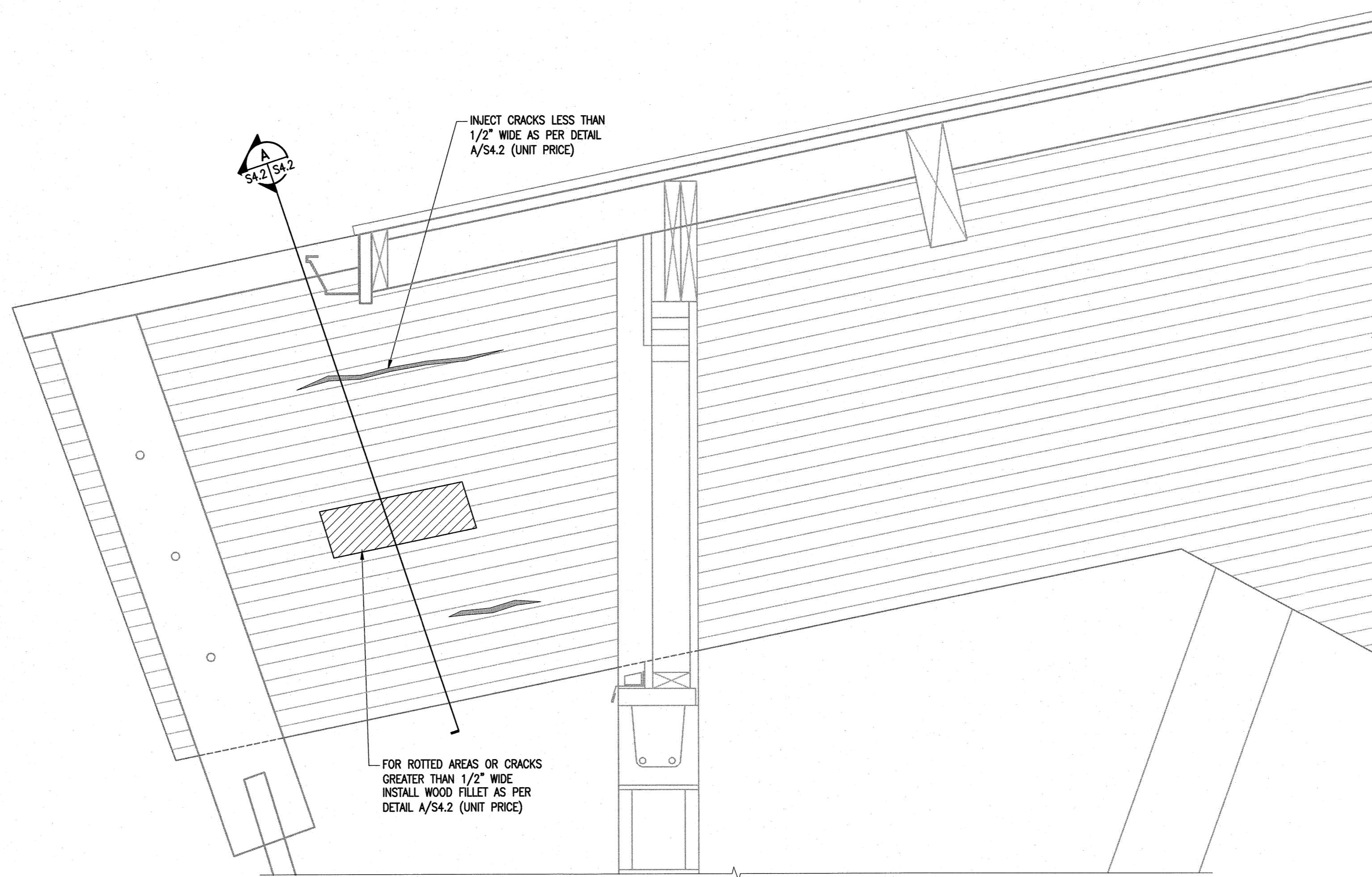
1 TYPICAL GLULAM ROT & CRACK REPAIR 1-1/2" = 1'-0"
