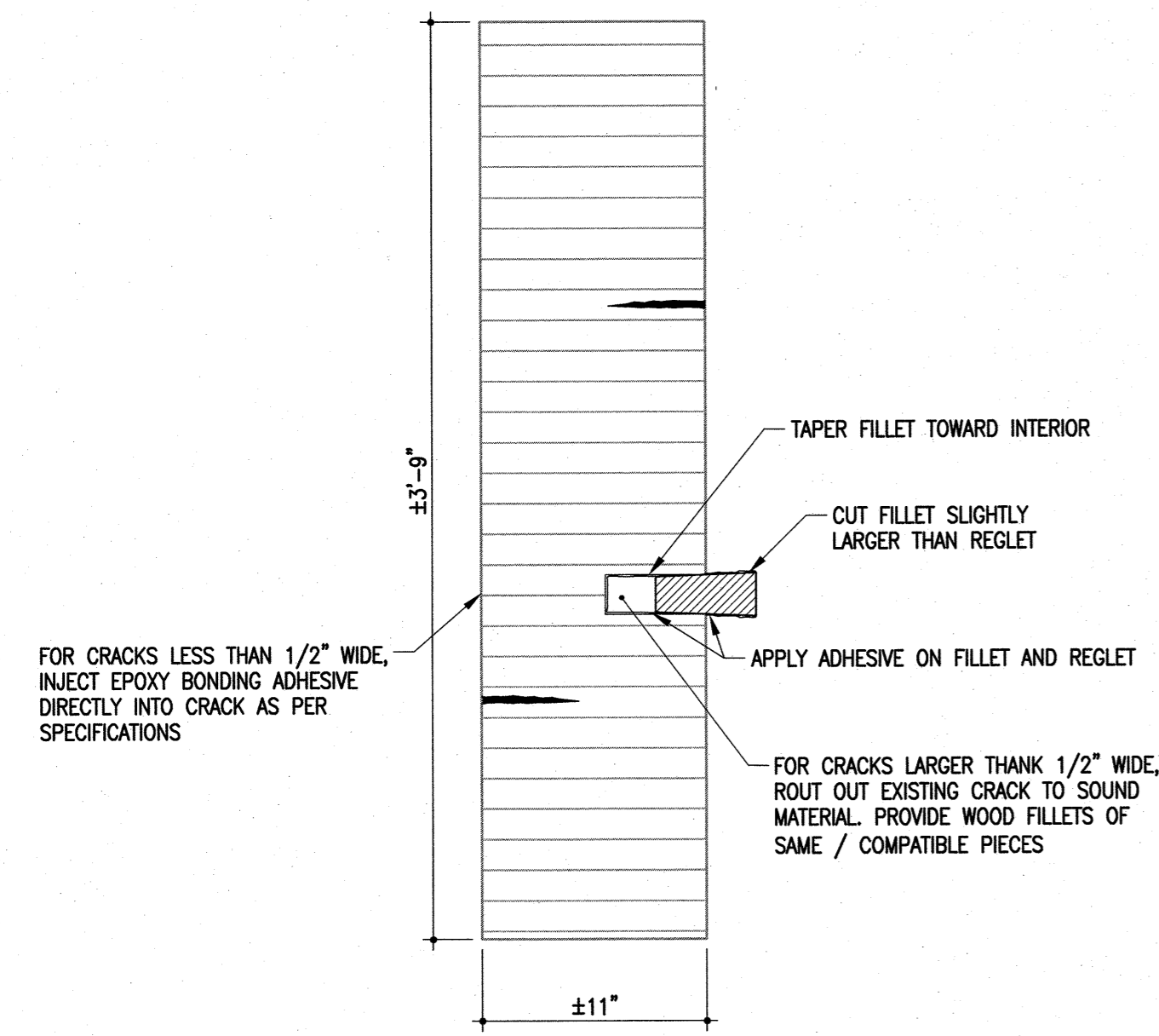
A EPOXY INJECTION & WOOD FILLET REPAIR SECTION 1-1/2" = 1'-0"
