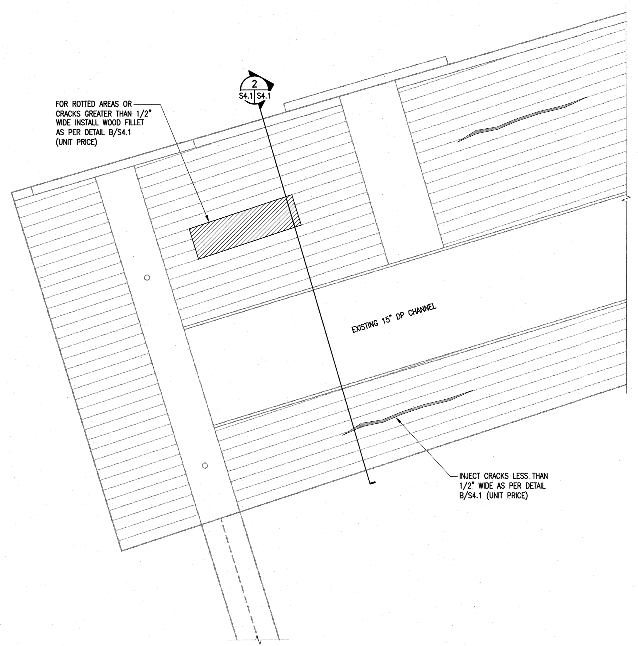
A PARTIAL GLULAM ELEVATION S4.1 1-1/2" = 1'-0"
