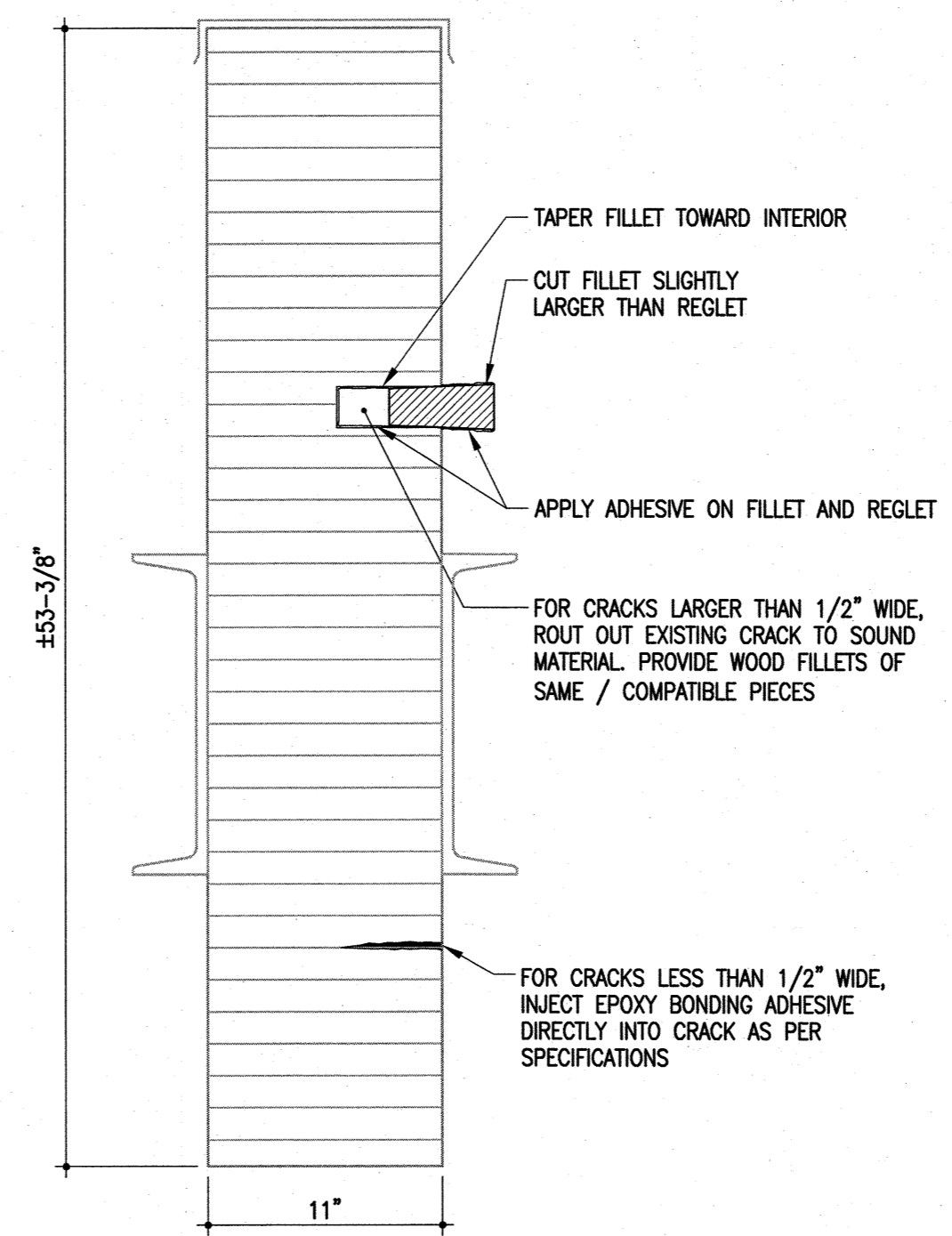
B GLULAM EPOXY INJECTION & WOOD FILLET REPAIR S4.1 S4.1 1-1/2" = 1'-0"
