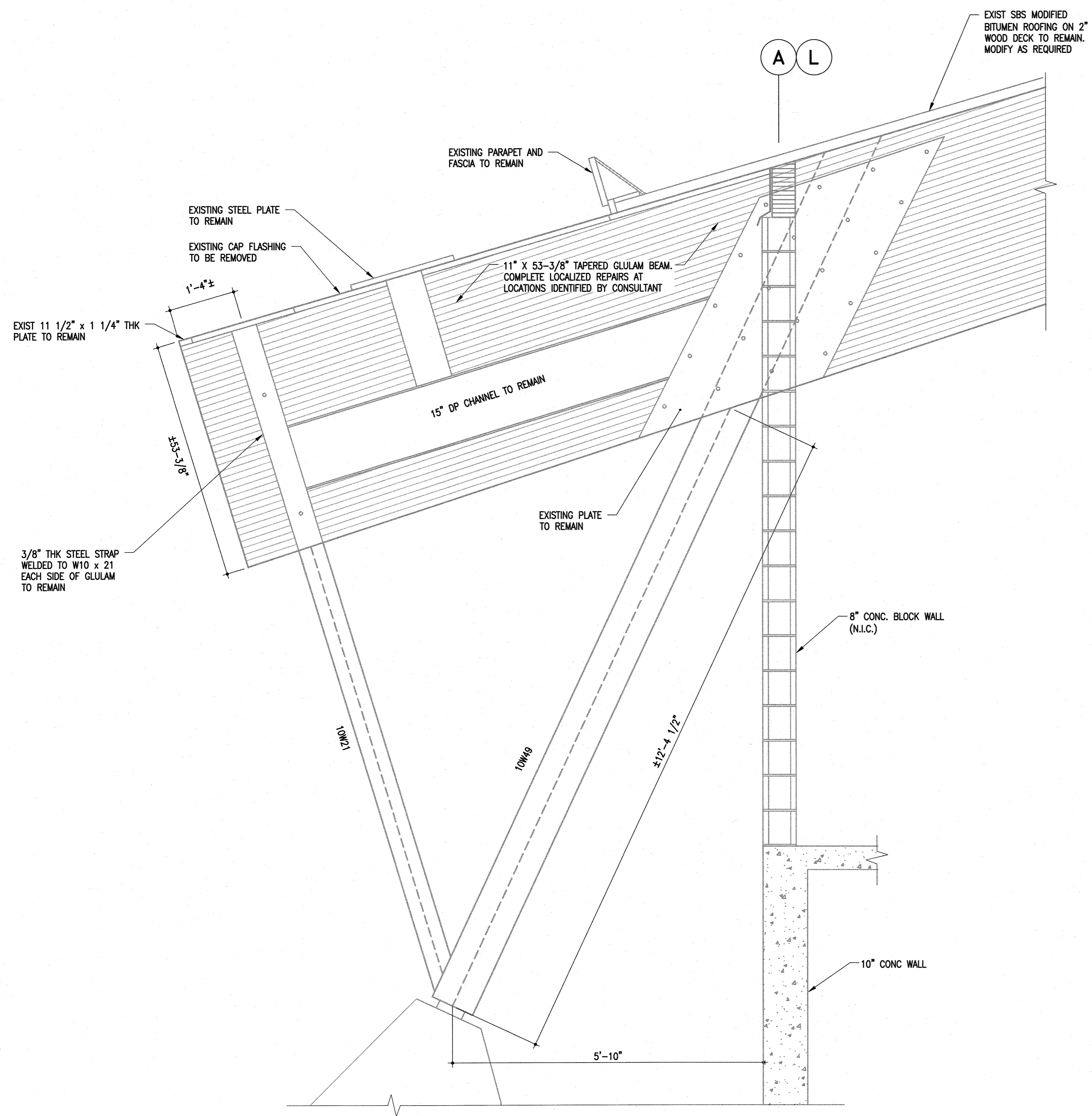
1 EXISTING TYPICAL GLULAM SECTION S2.1 S4.1 3/4" = 1'-0"
