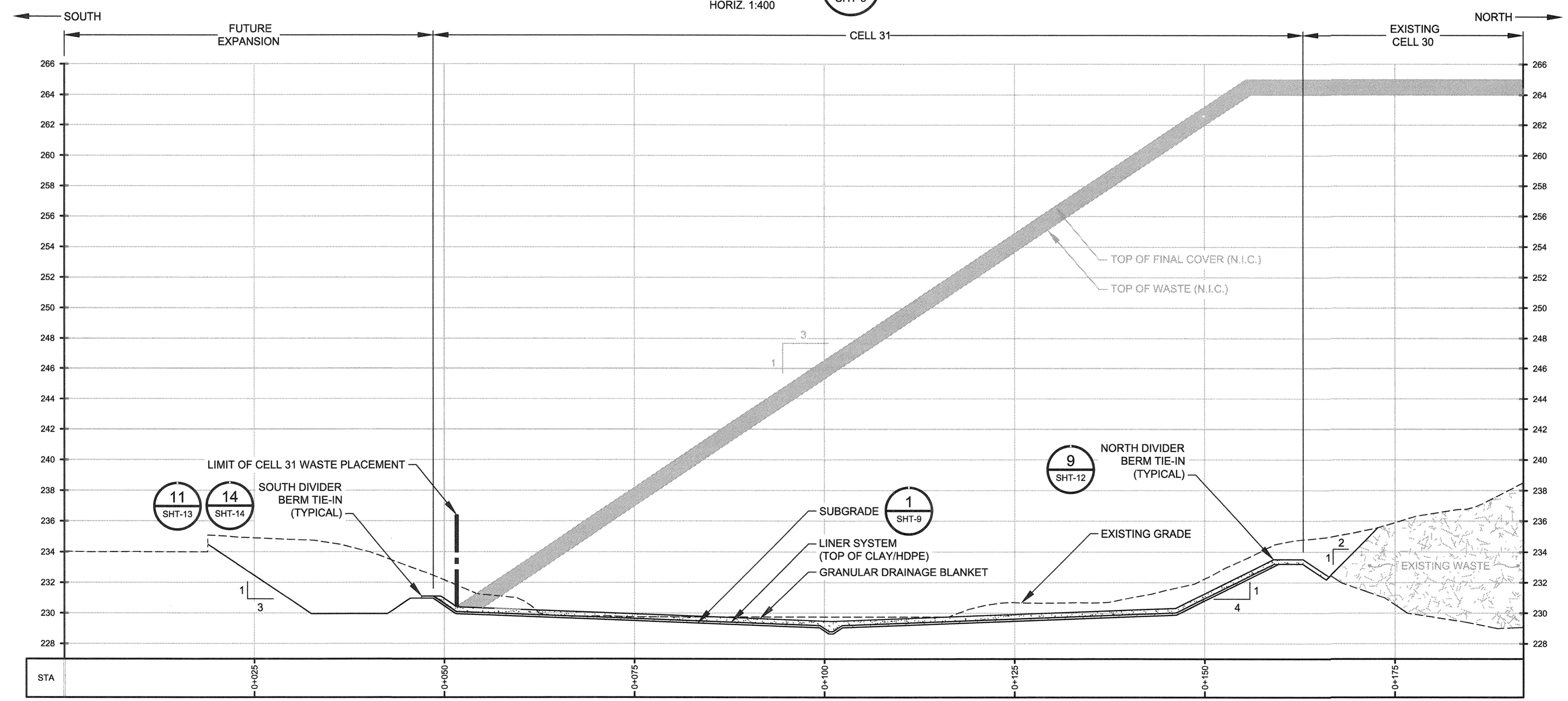
SECTION B-B VERT: 1:200 HORIZ: 1:400 SHT-5
