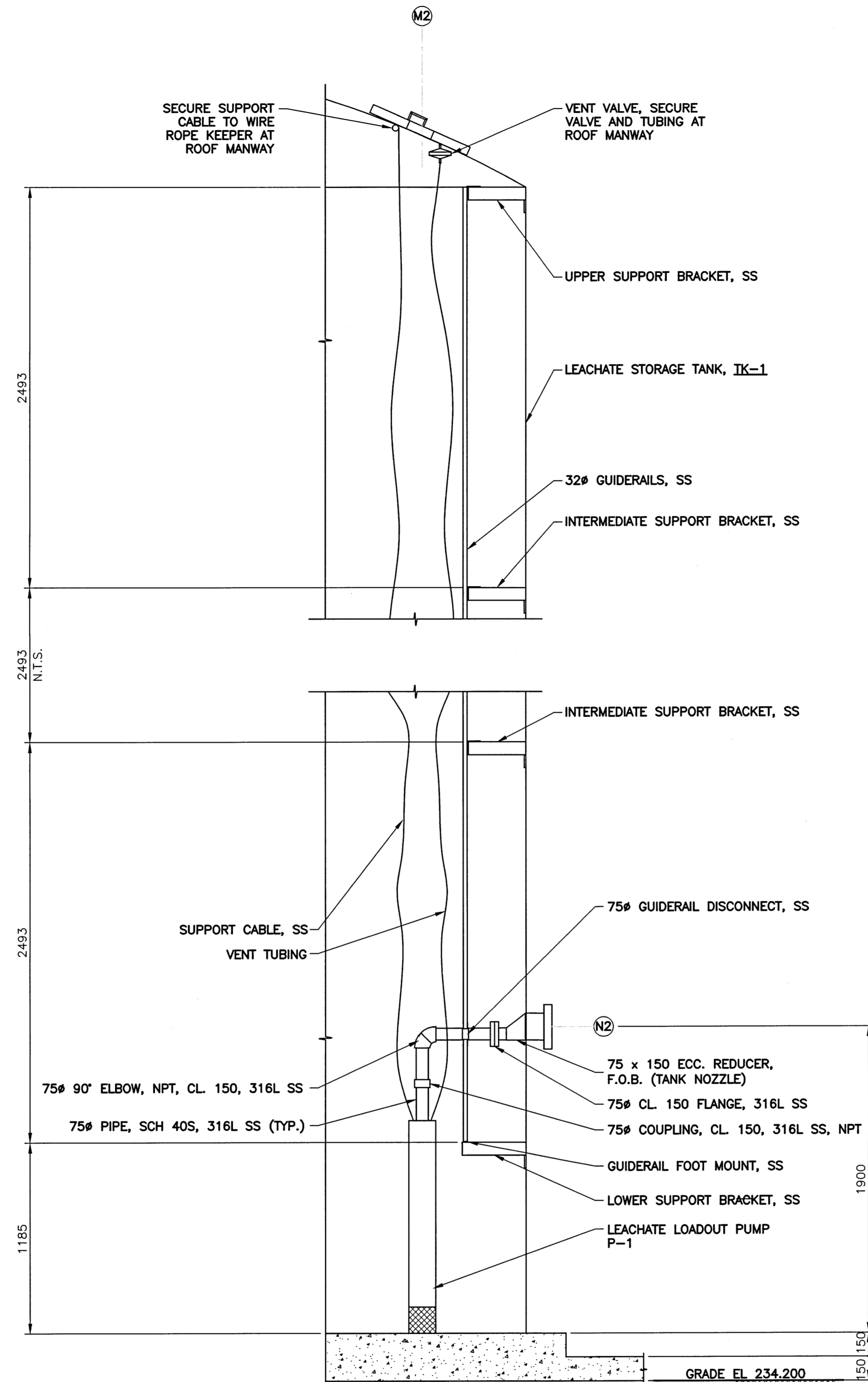
1 DETAIL - LEACHATE LOADOUT PUMP
