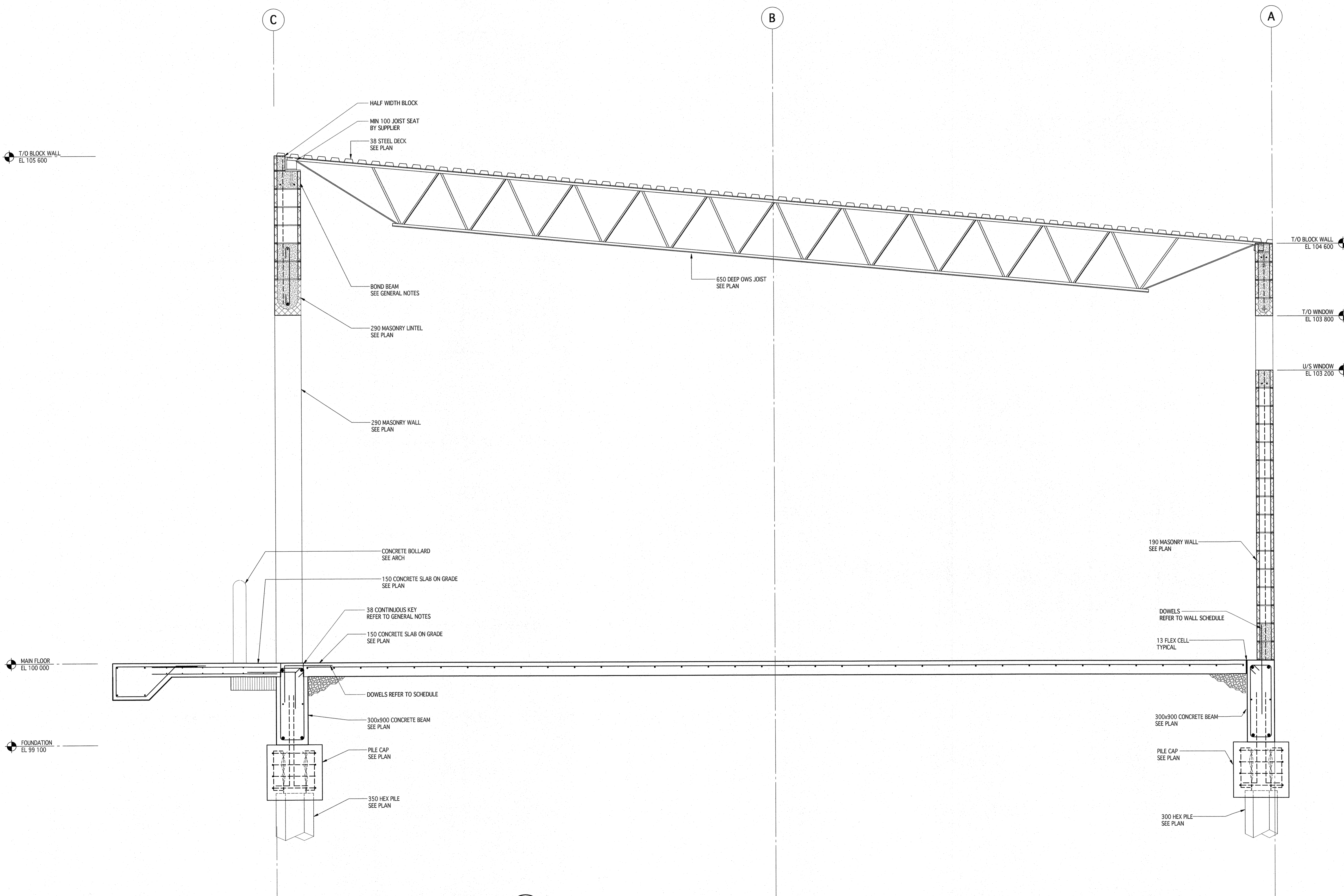
1 SECTION FH | S4.2 1:20
