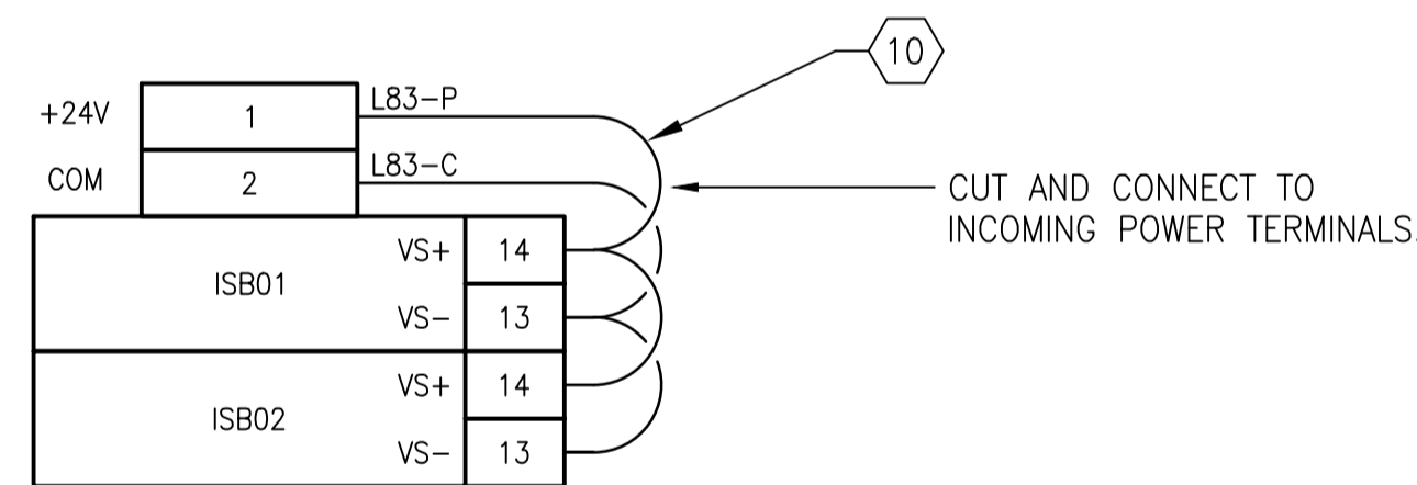
DETAIL: POWER BUS CONNECTION
