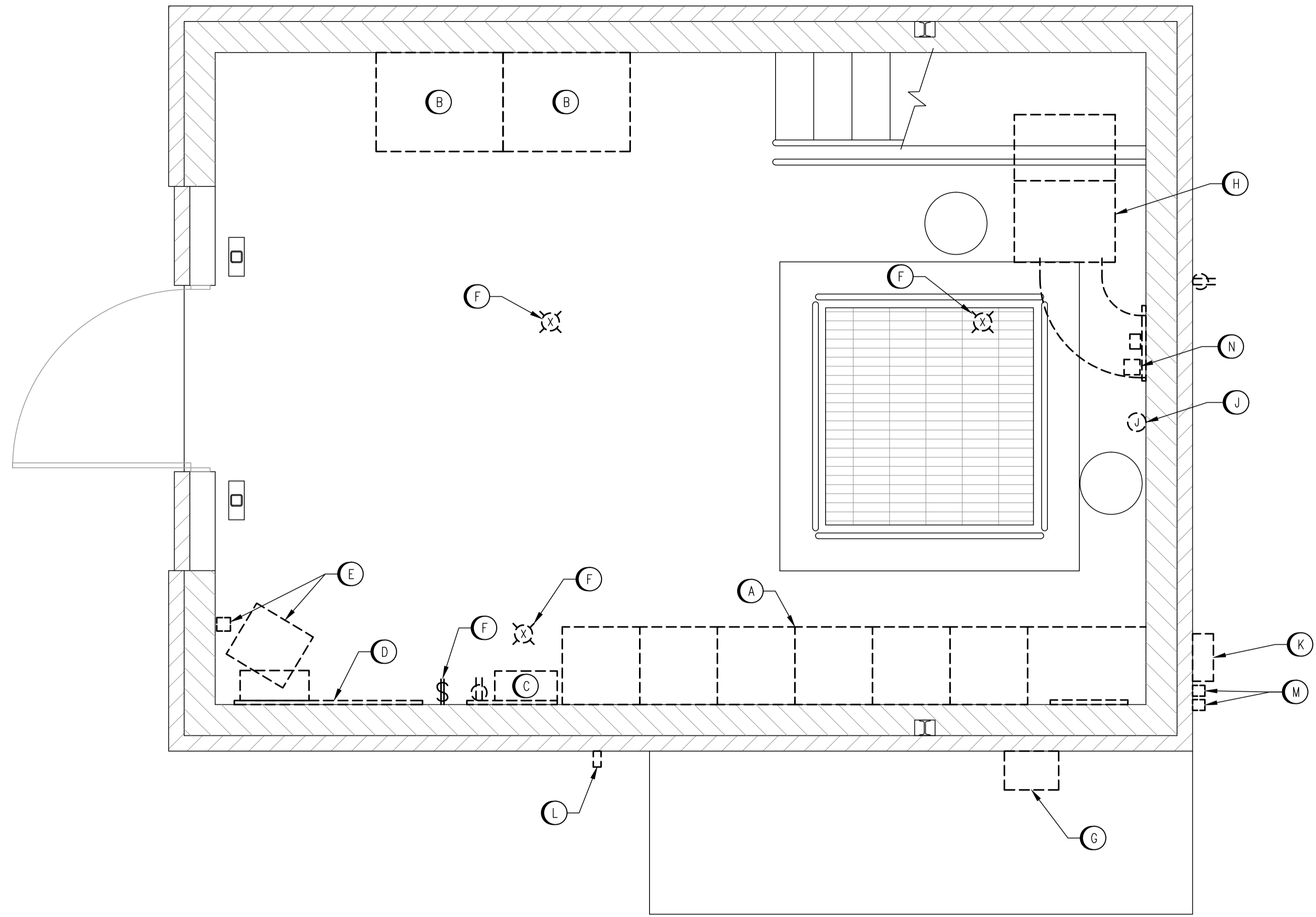
MAIN FLOOR PLAN SCALE: 1 : 20
