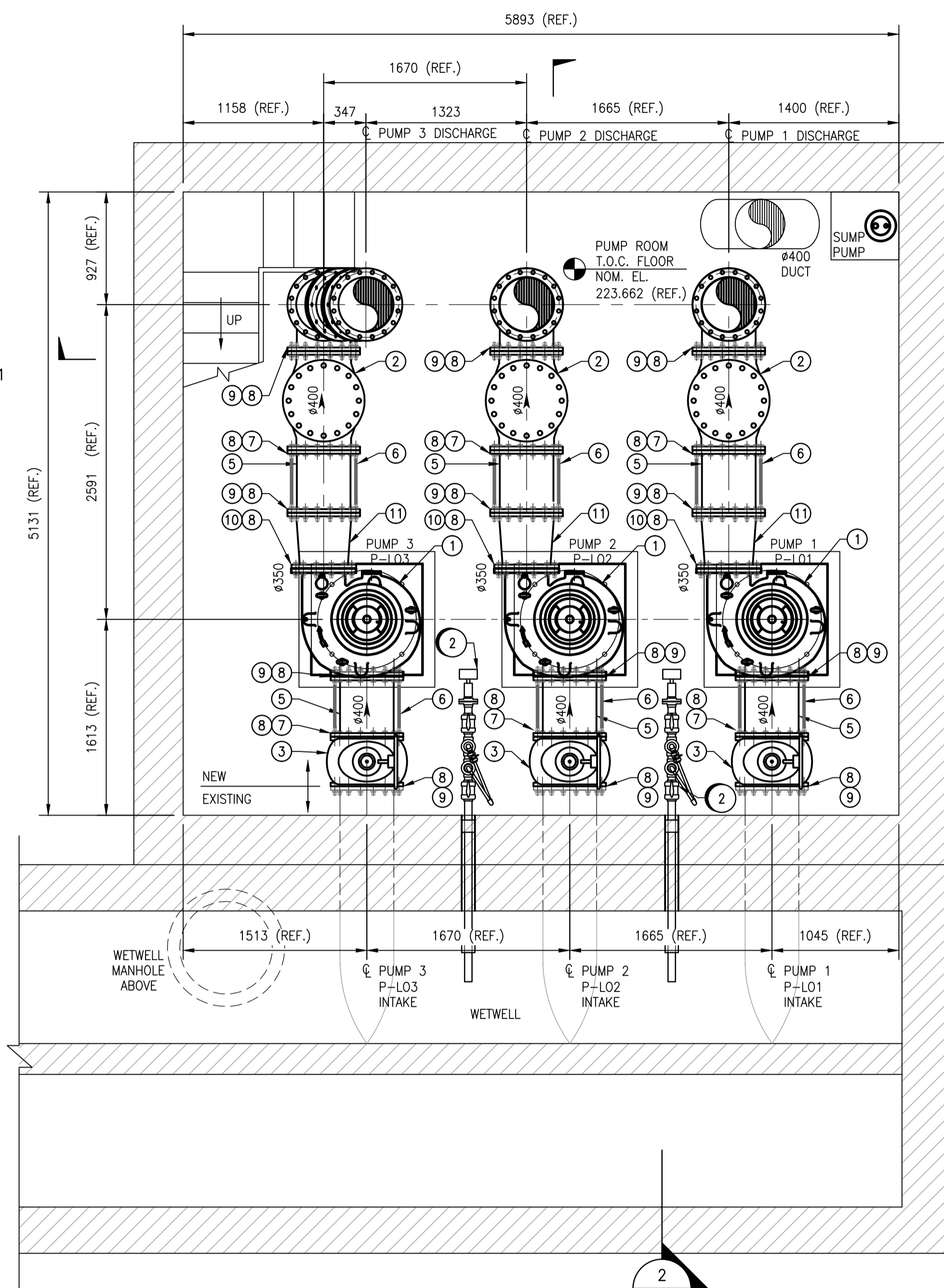
SUMP ROOM FLOOR PLAN - NEW WORK SCALE: 1 : 30
