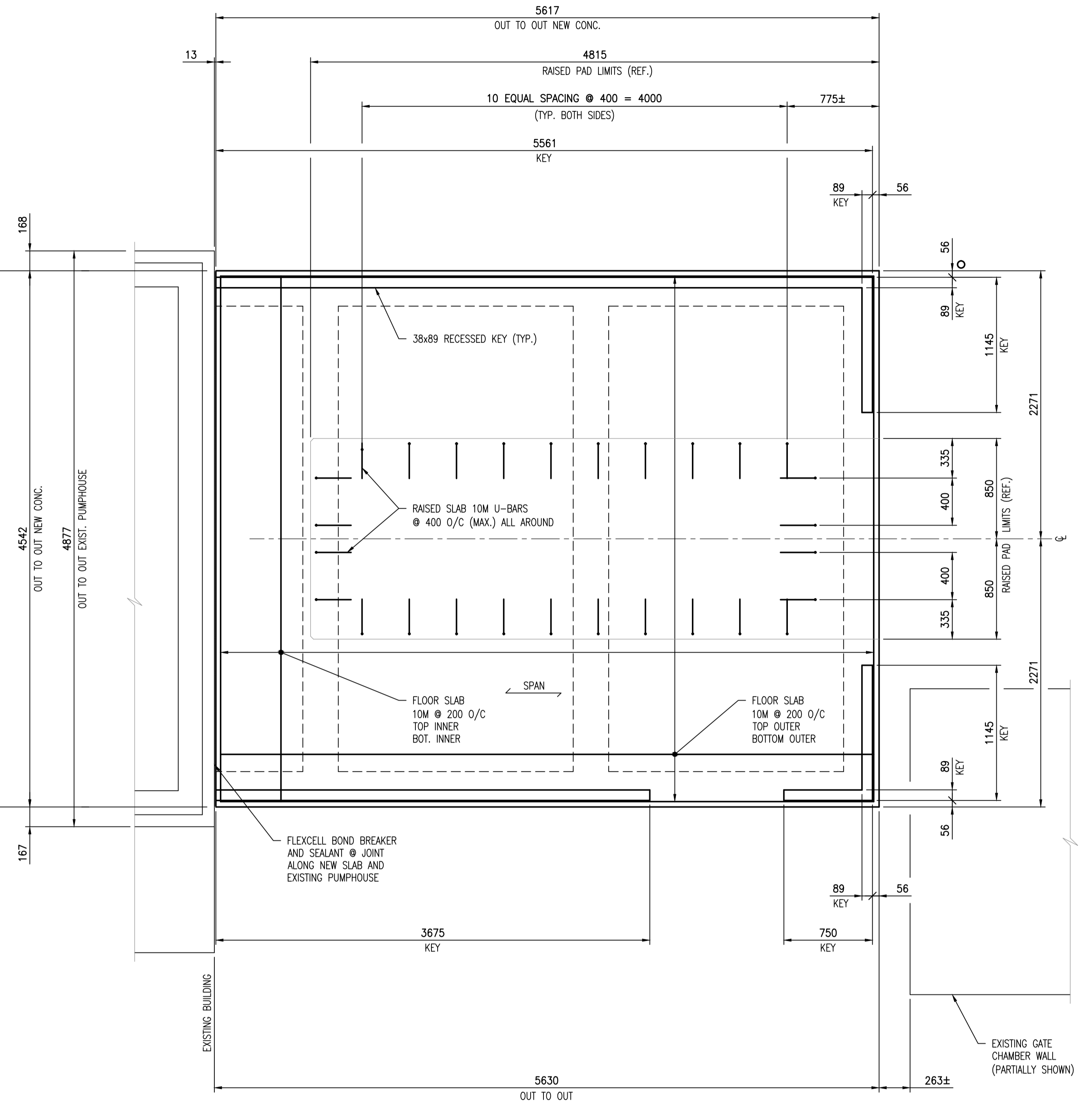
PLAN - STRUCTURAL FLOOR SLAB 1 : 25
