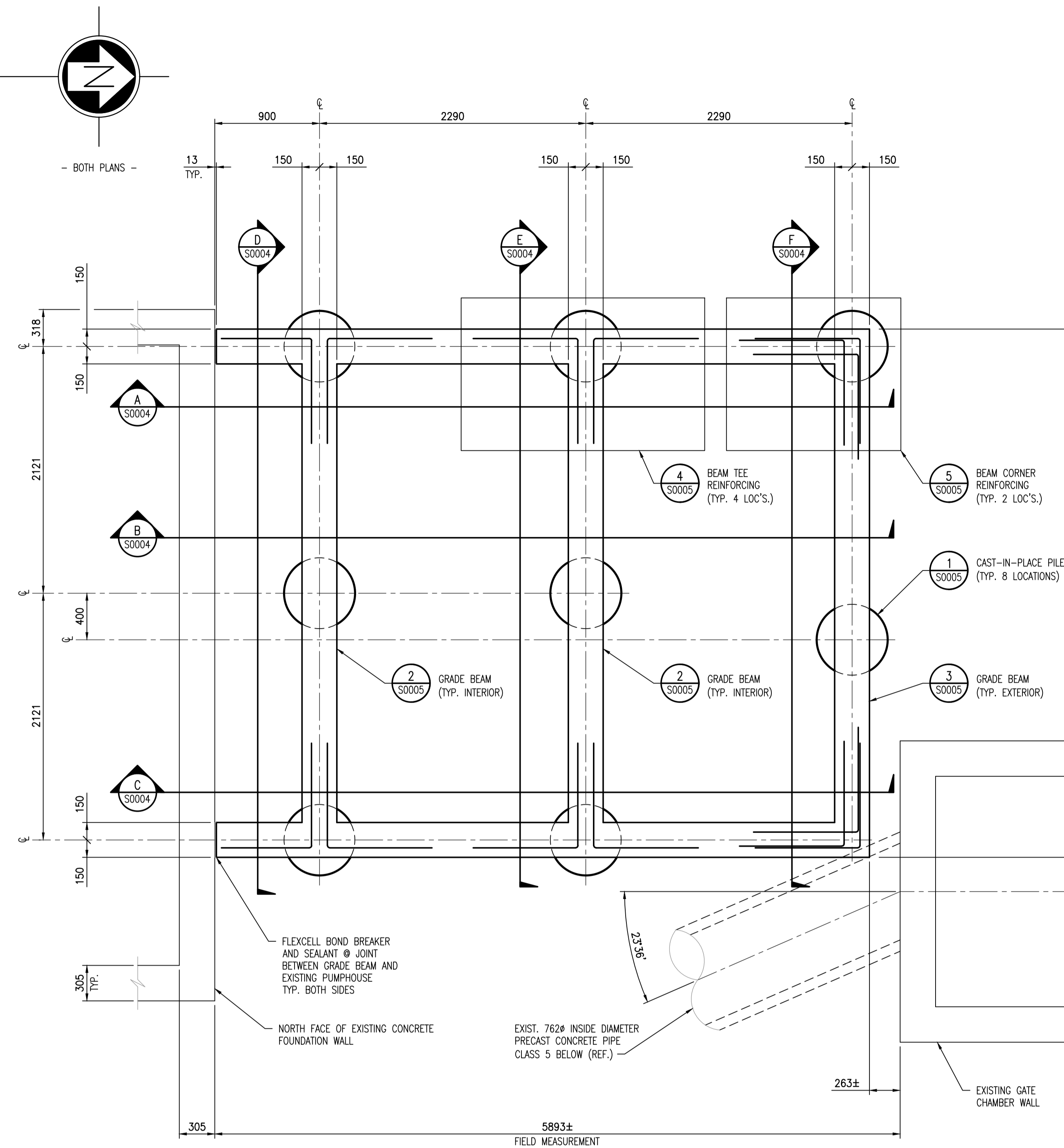
FOUNDATION/PILE PLAN 1 : 25
