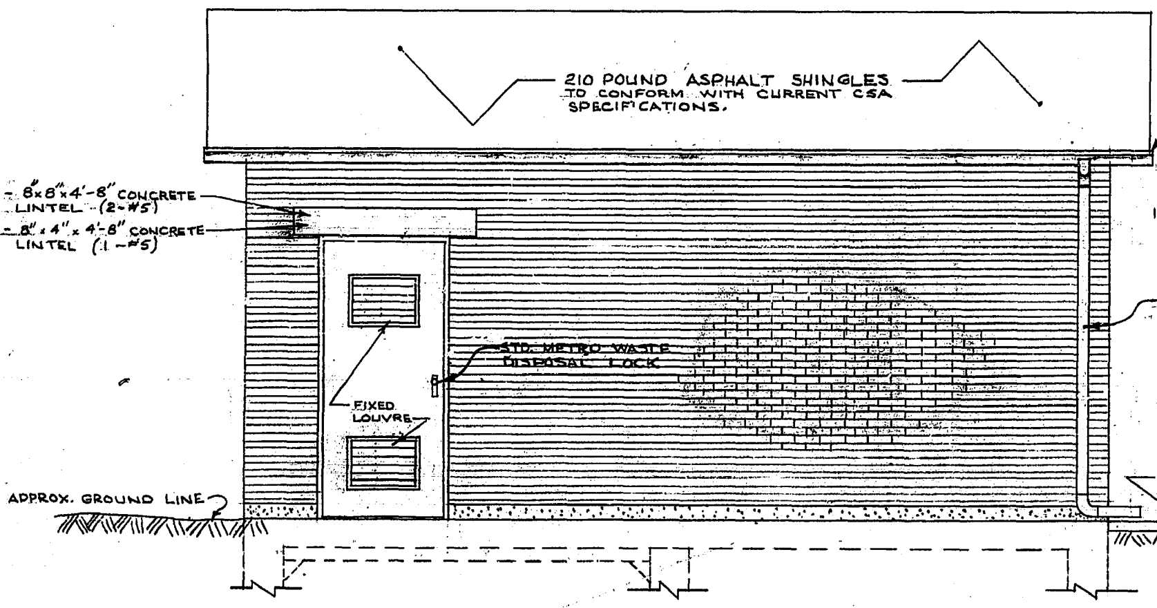
EAST WALL ELEVATION SCALE: 3/8" = 1'-0"
