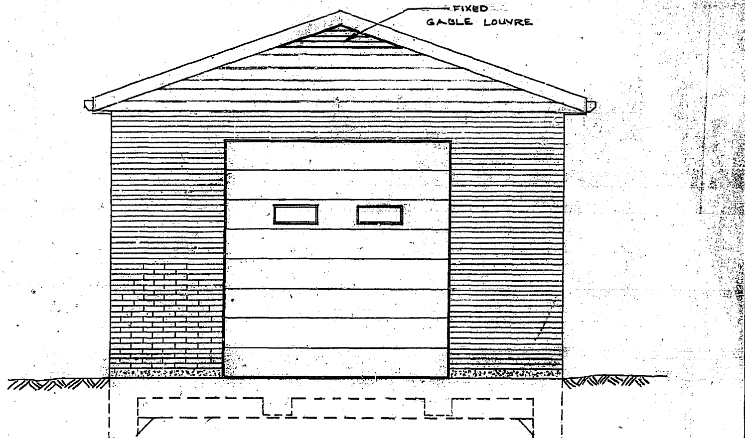
SOUTH WALL ELEVATION SCALE: 3/8" = 1'-0"
