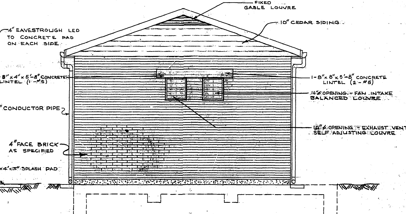
NORTH WALL ELEVATION SCALE: 3/8" = 1'-0"
