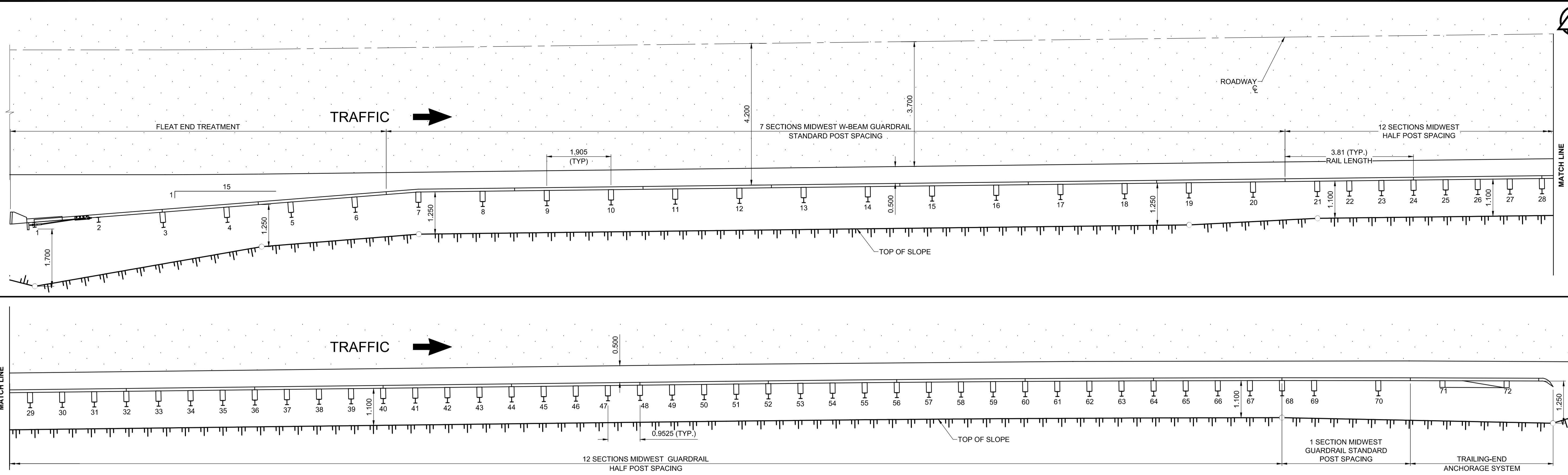
SOUTH GUARDRAIL LAYOUT PLAN 1:100
