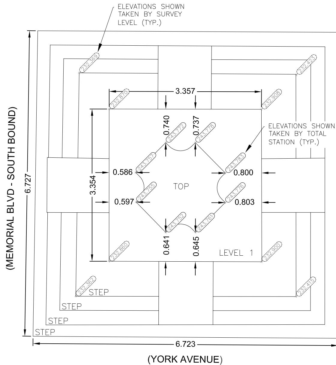
PLAN VIEW 1:50
