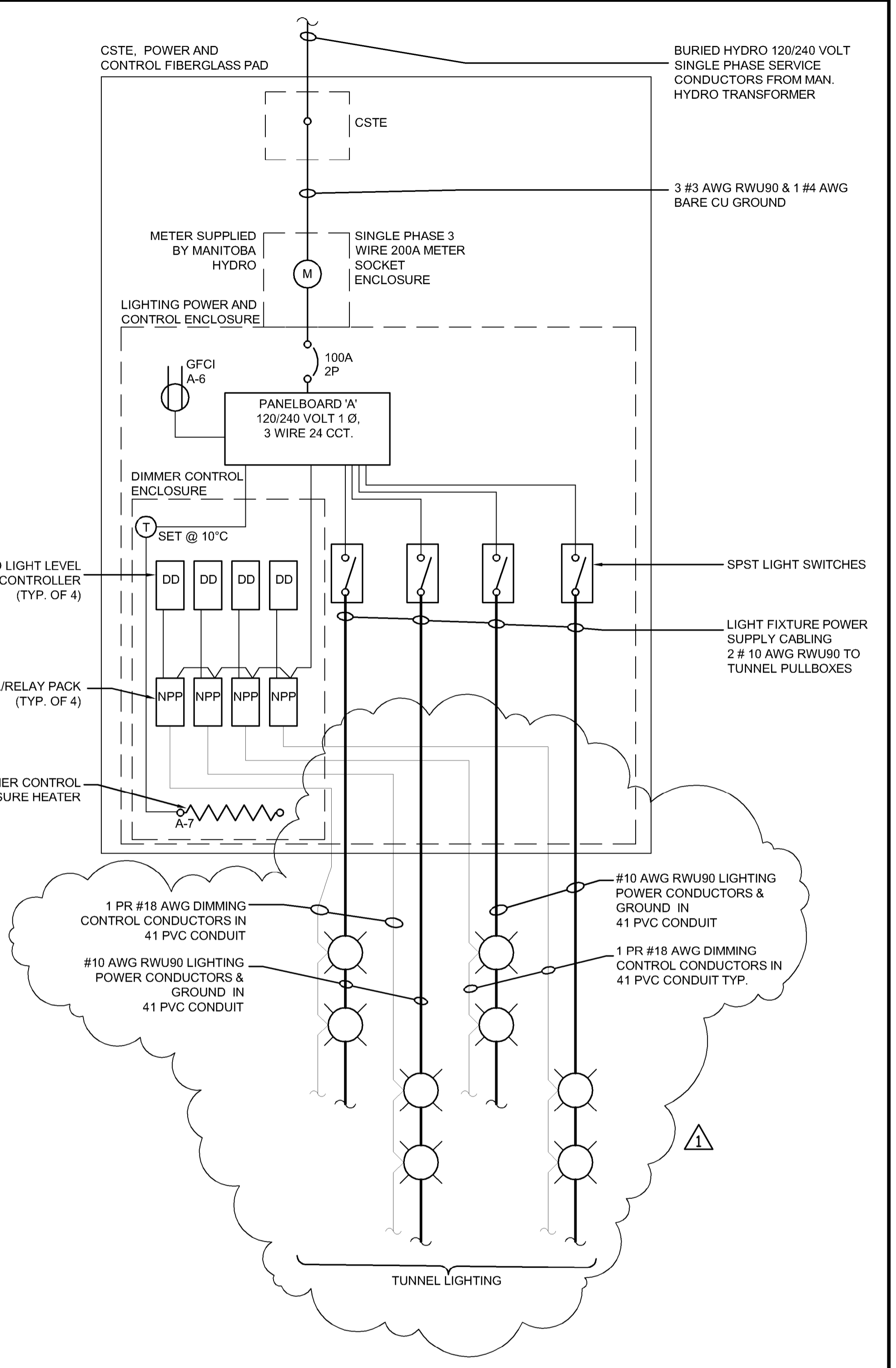
SINGLE LINE DIAGRAM
