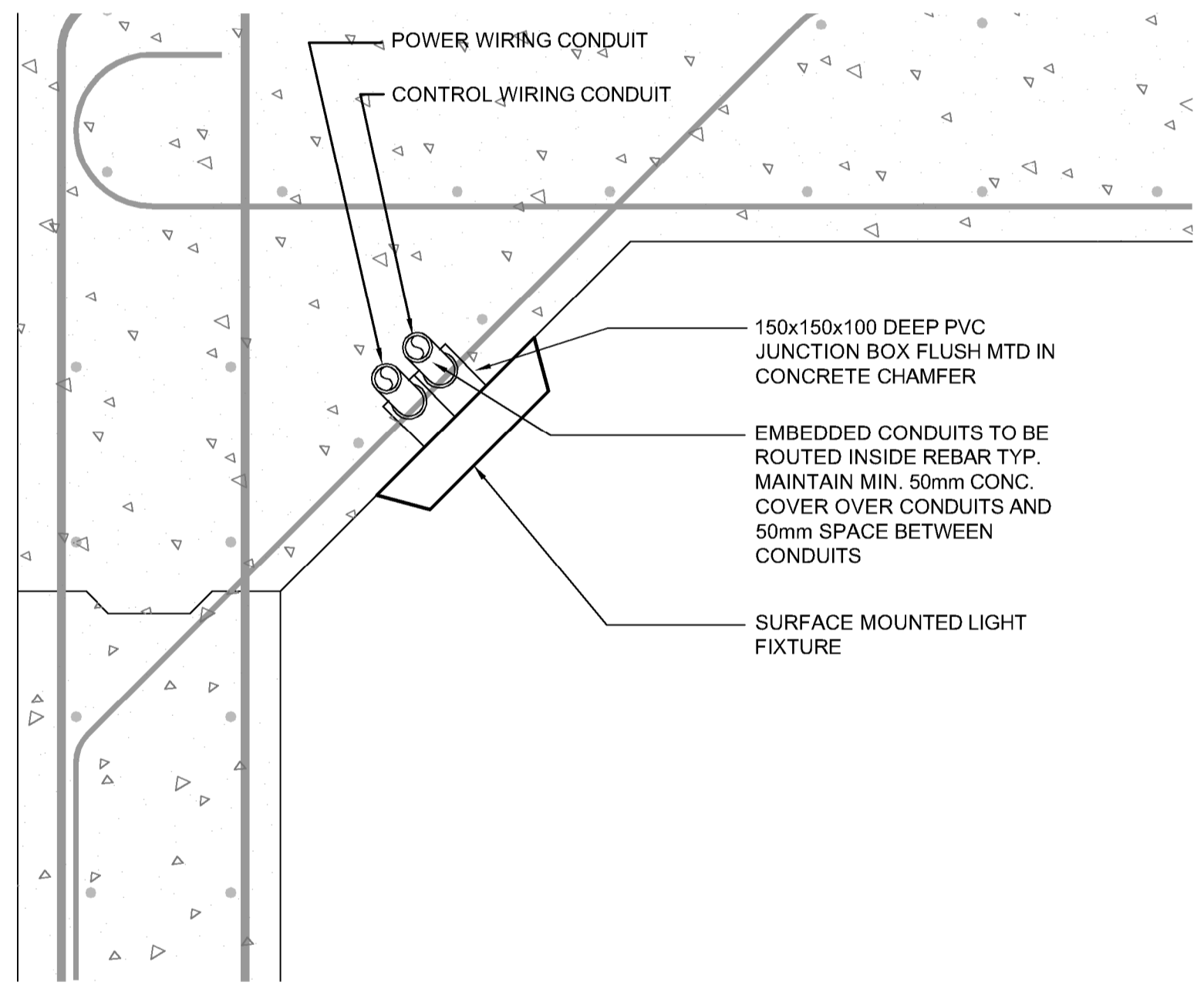
E TUNNEL LIGHT FIXTURE MOUNTING DETAIL N.T.S.
