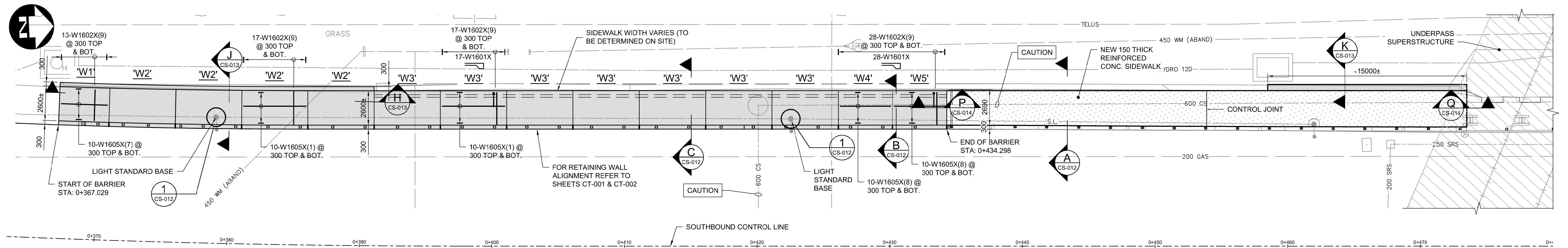
SOUTHWEST SIDEWALK RECONSTRUCTION - PLAN 1:150
