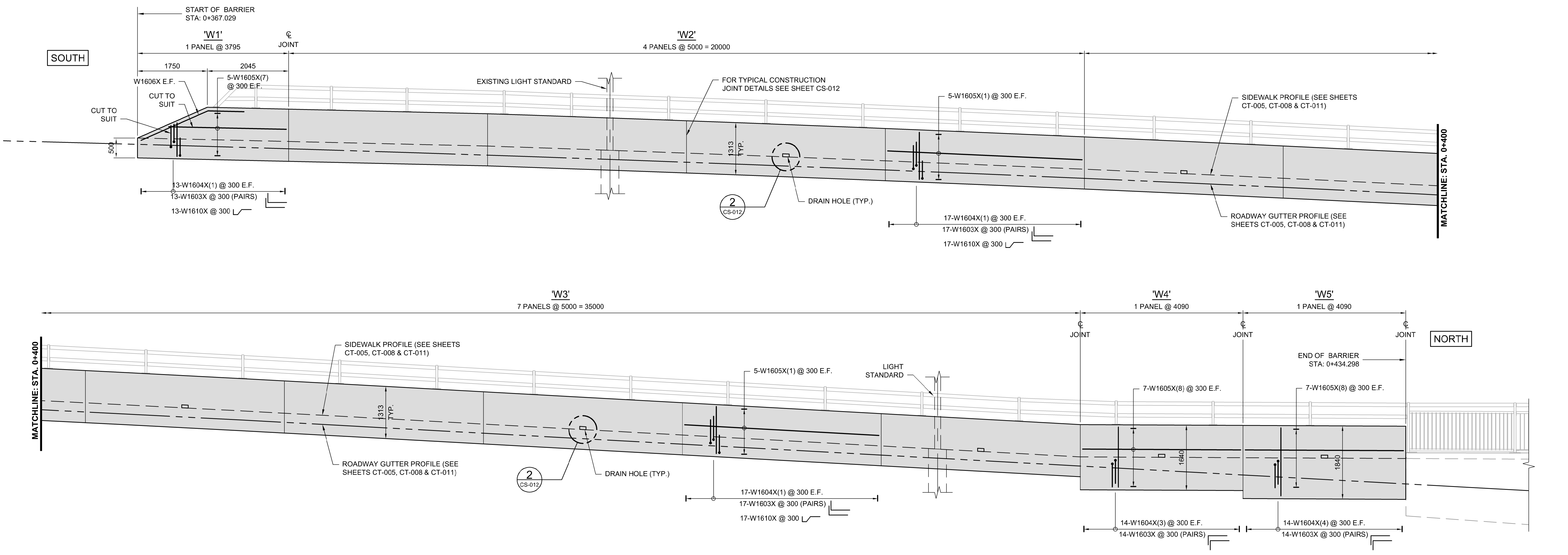
SOUTHWEST SIDEWALK RECONSTRUCTION - ELEVATION 1:50
