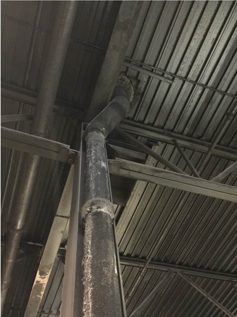
TYPICAL EXISTING DRAIN LINE
