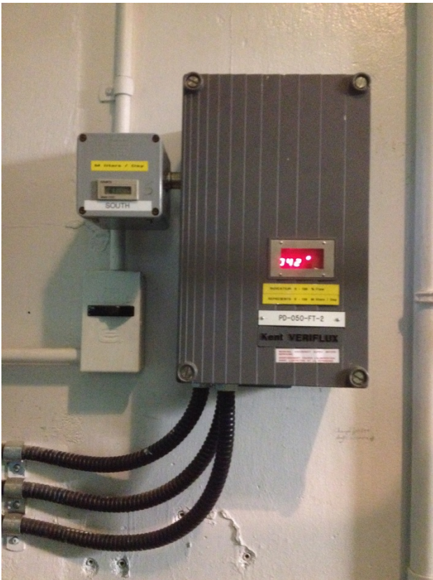
Photo 5: McPhillips Pumping Station Flow Meter Transmitter
