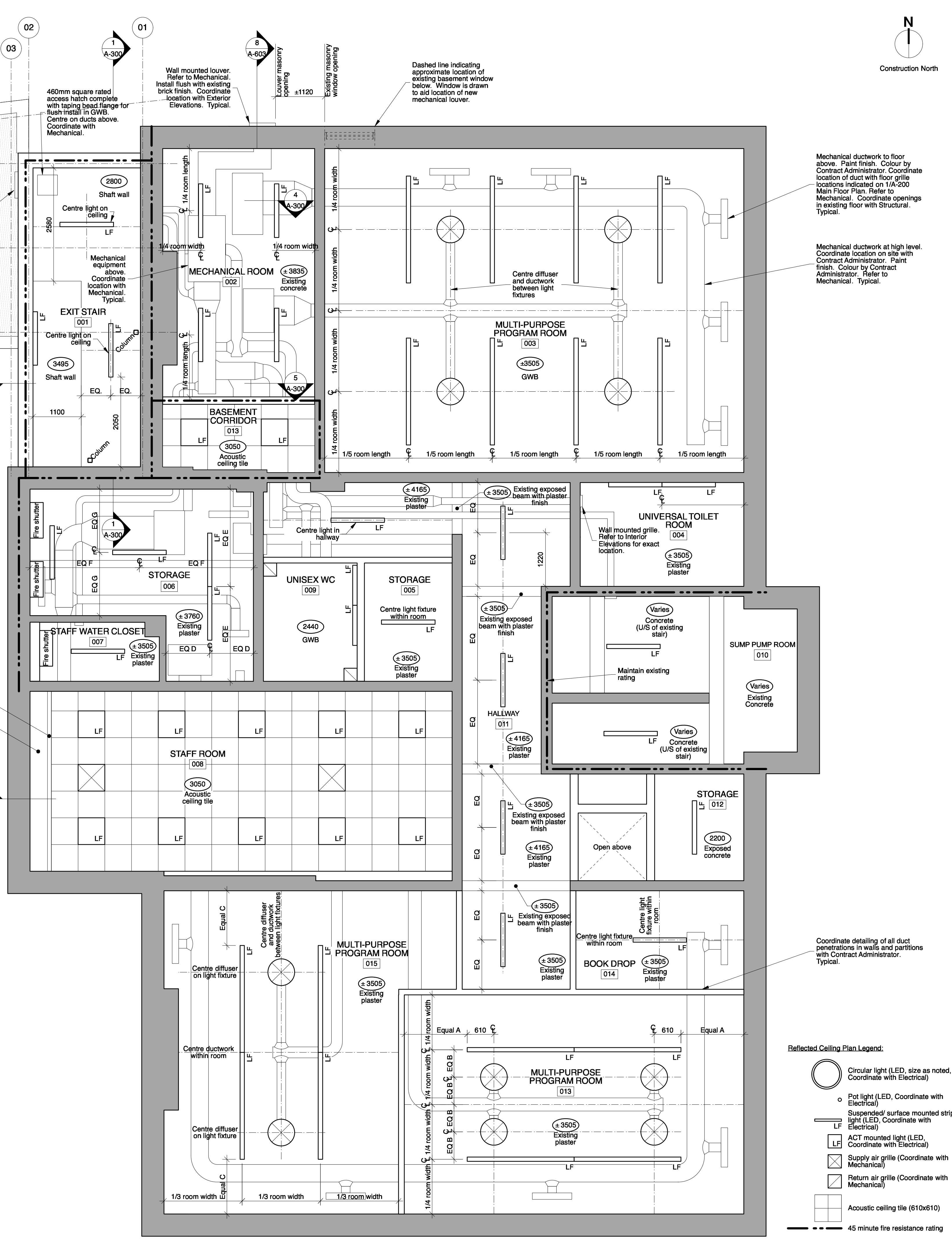
1 Basement Reflected Ceiling Plan A-204 1:50
