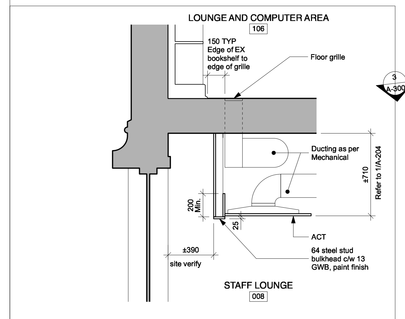
2 Section Thru Staff Lounge 008 Ceiling Bulkhead A-204 1:20
