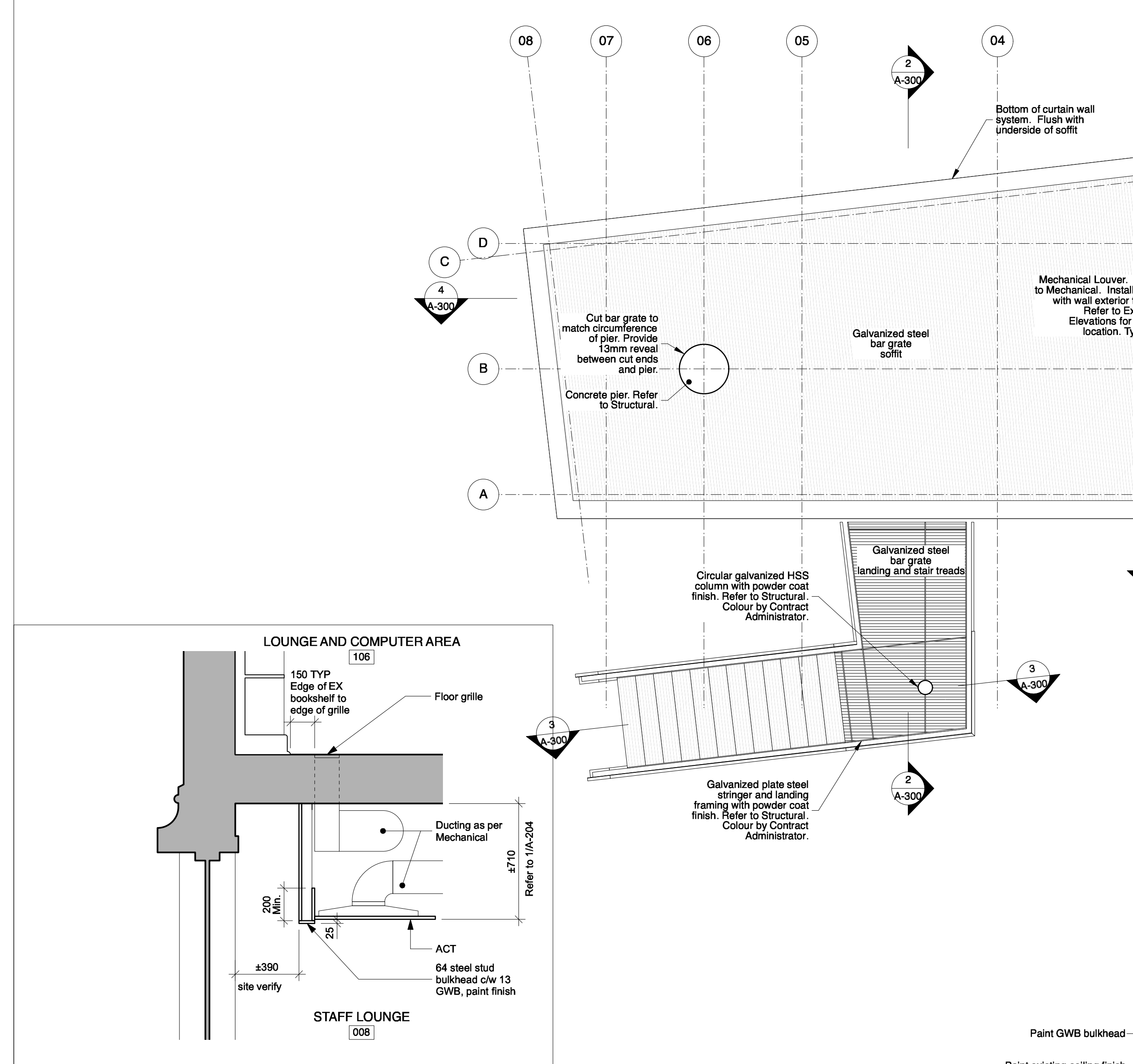
2 Section Thru Staff Lounge 008 Ceiling Bulkhead A-204 1:20
