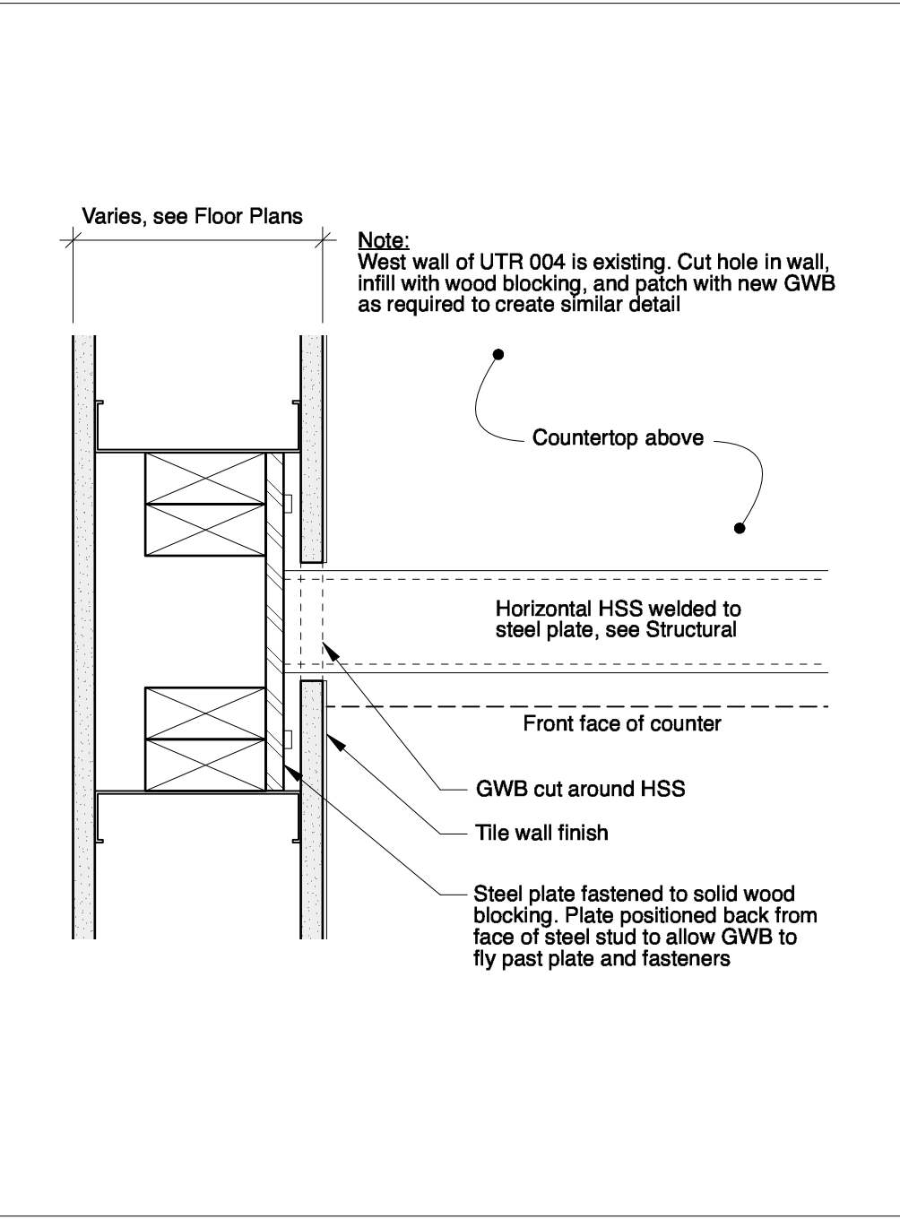
9 Plan Detail - UTR Lavatory Counter at Side Wall A-700 1:5
