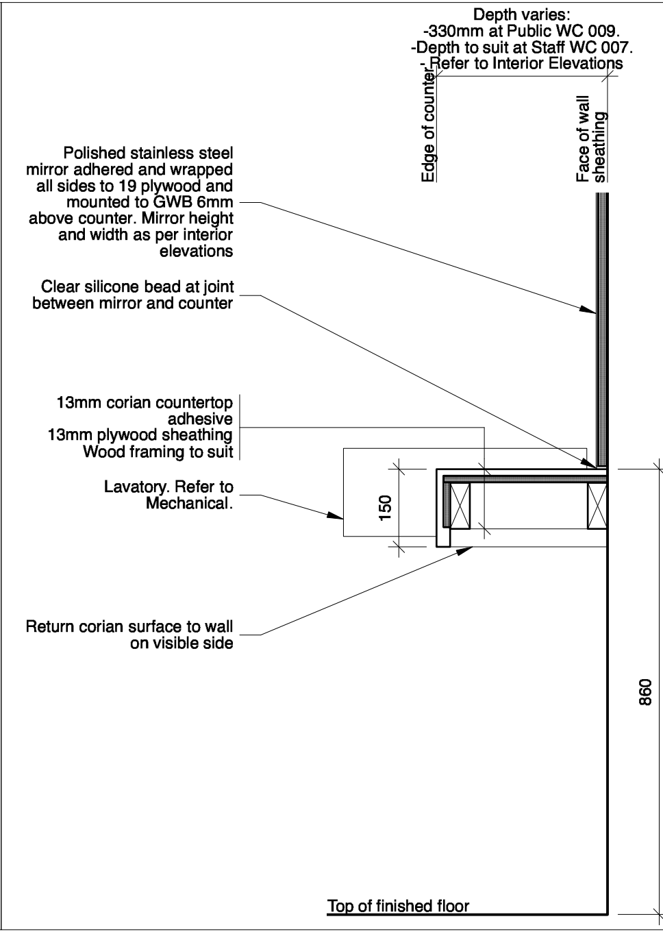
2 Section Detail - Lavatory Counter A-700 1:10
