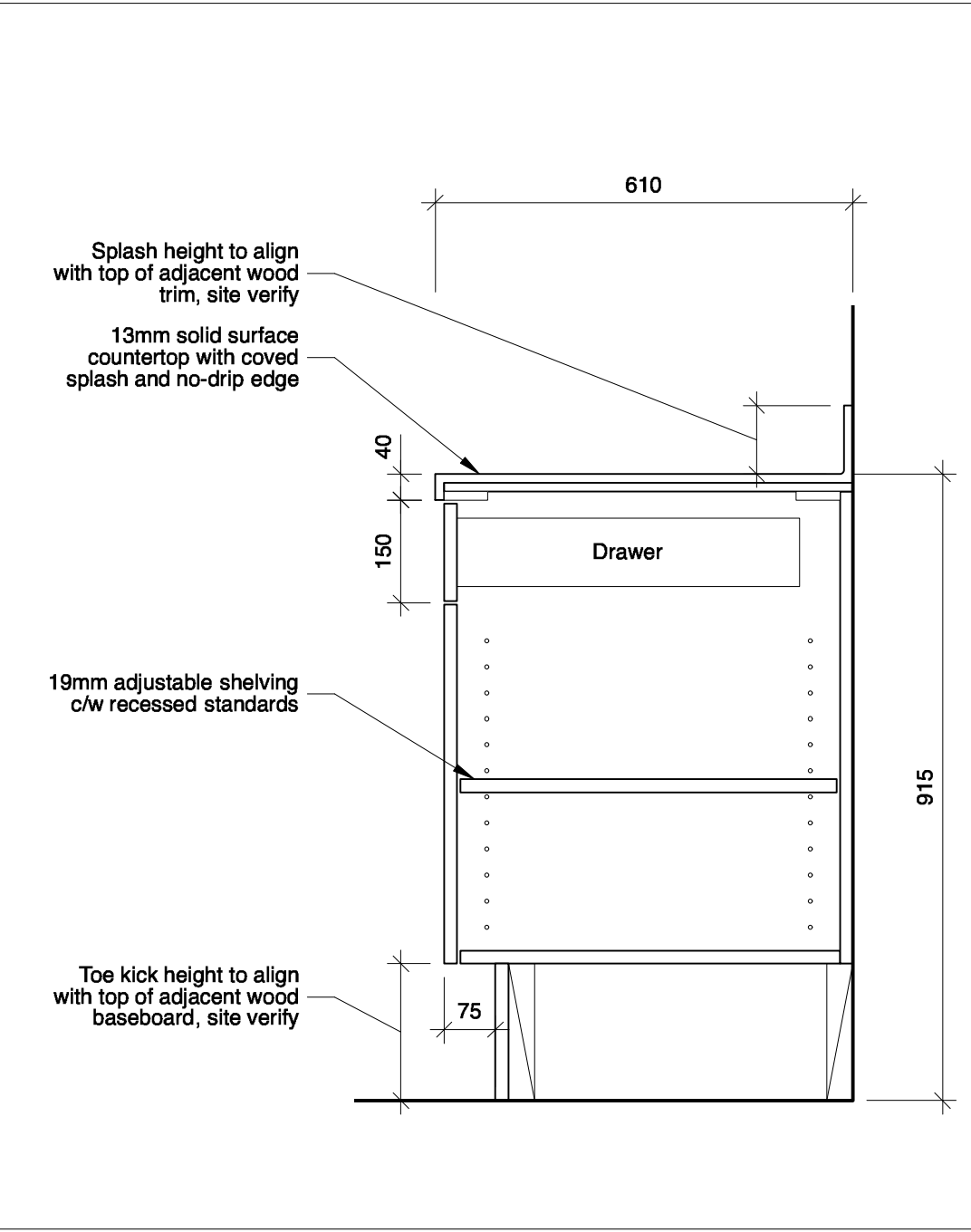
8 Section Detail - Staff Room Millwork A-700 1:10
