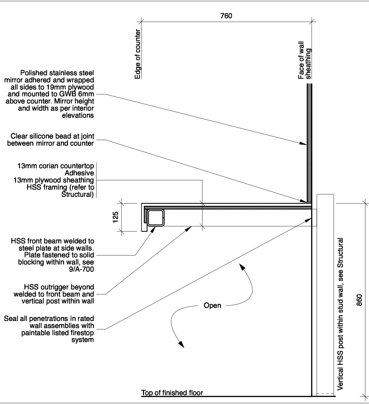
1 Section Detail - UTR Lavatory Counter A-700 1:10
