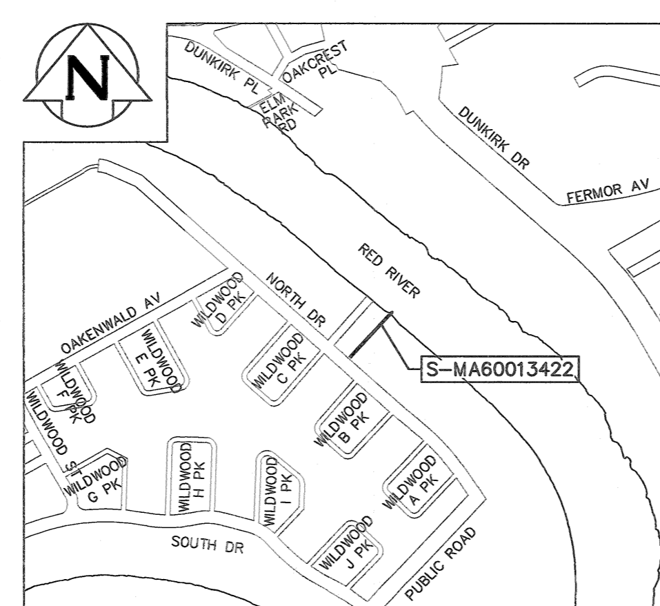
NORTH DRIVE OUTFALL
