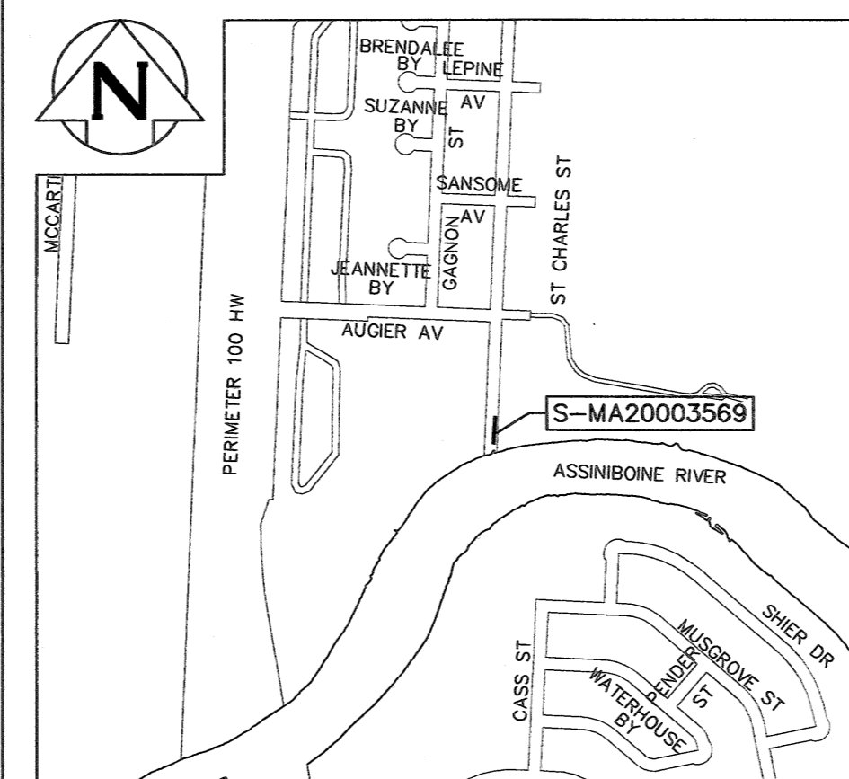
ST CHARLES STREET OUTFALL
