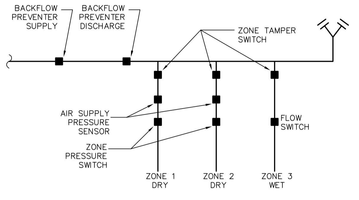
2 WATERMAIN RISER DIAGRAM
