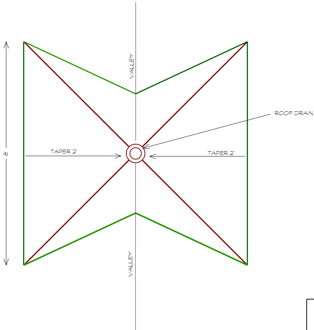
8" x 8" ROOF DRAIN SUMP DETAIL
