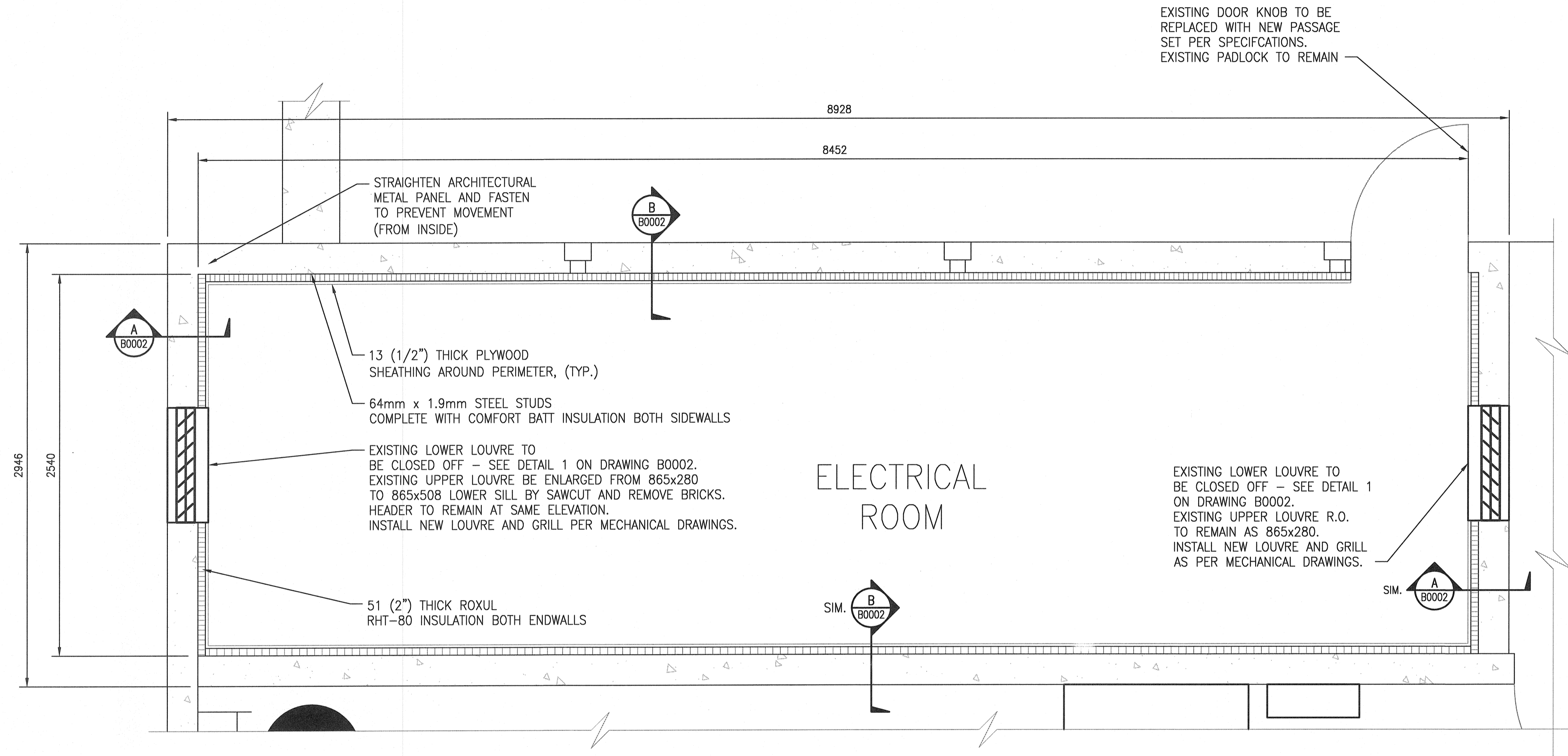
PARTIAL MAIN FLOOR PLAN SCALE: 1 : 20
