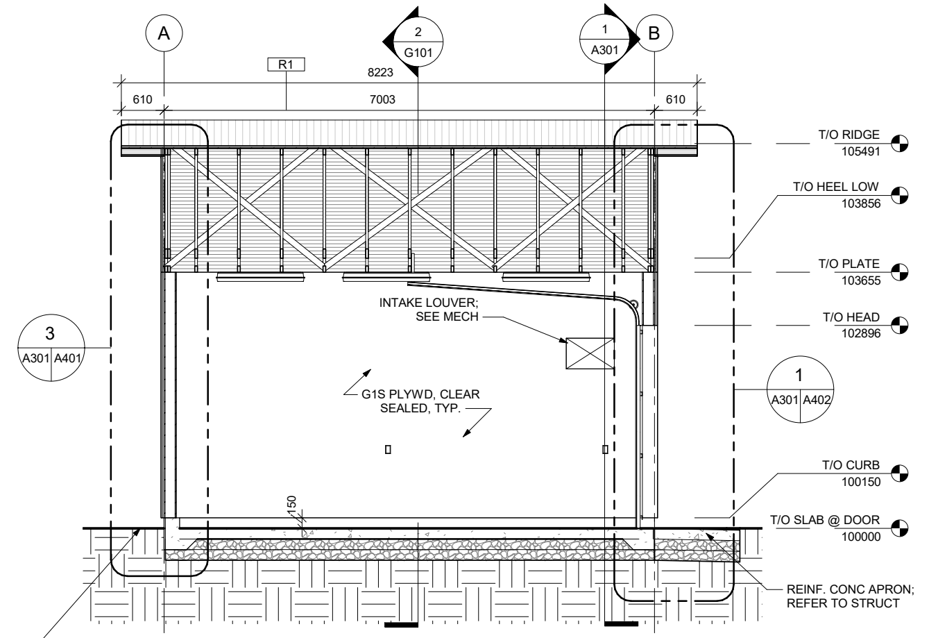
2 BUILDING SECTION 2 1:75
