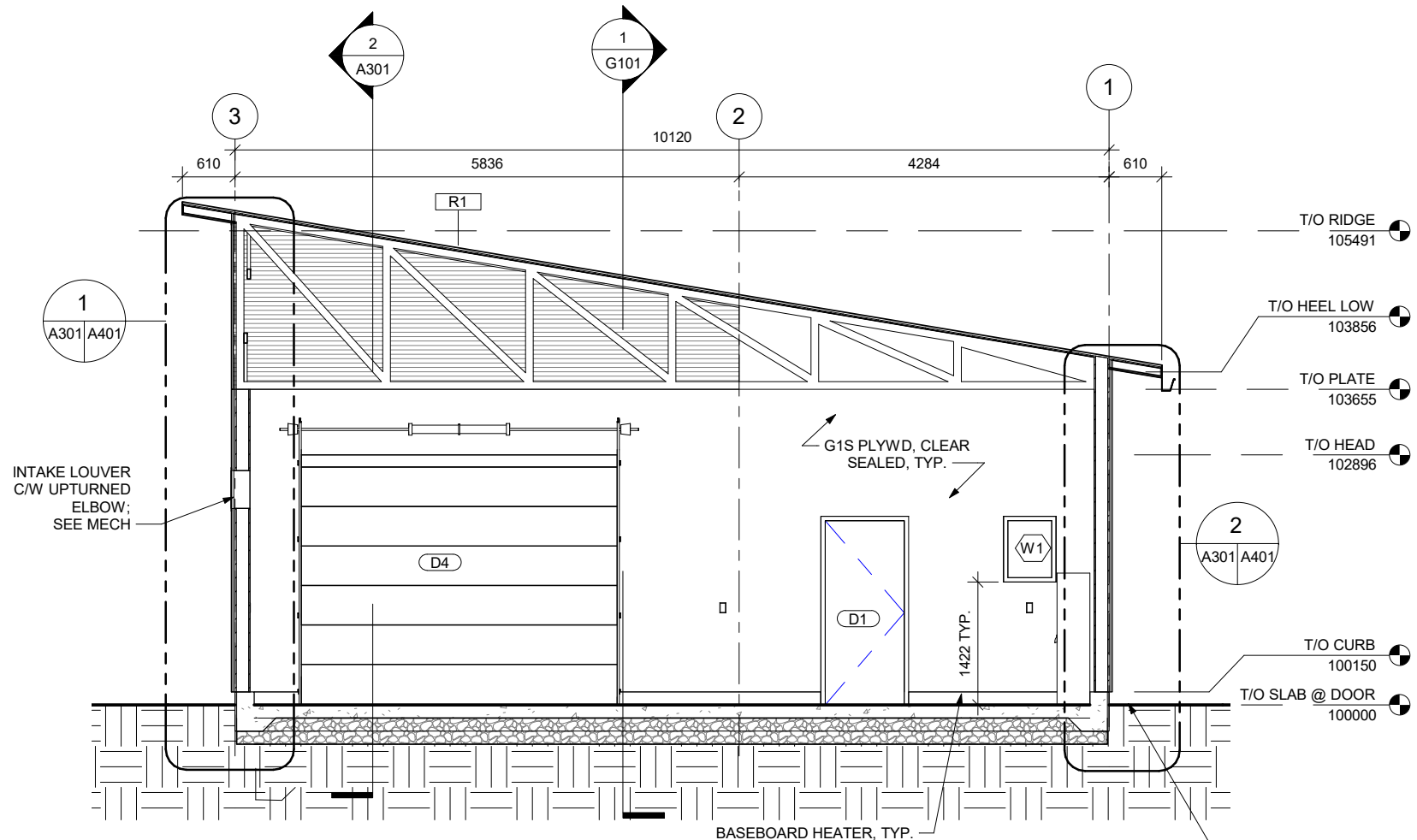
1 BUILDING SECTION 1 1:75
