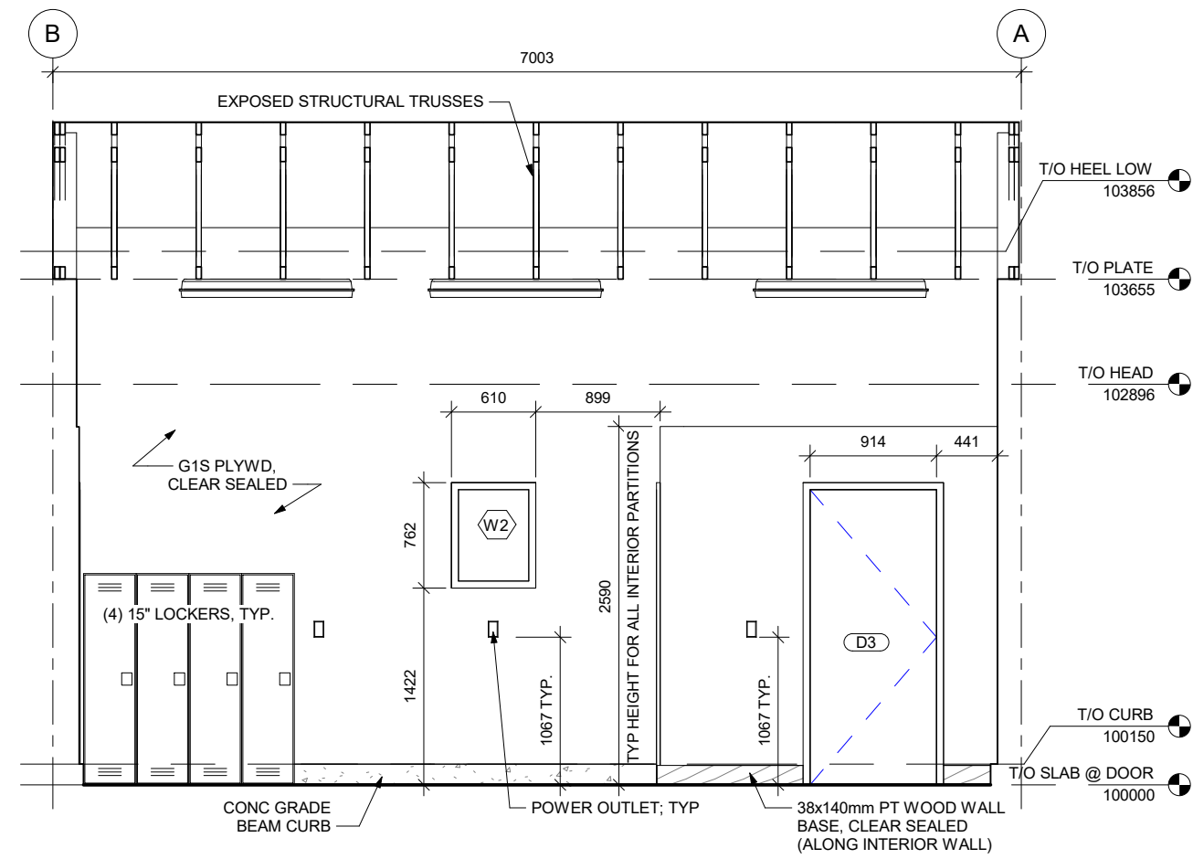
2 INT ELEVATION - GARAGE - D 1:50
