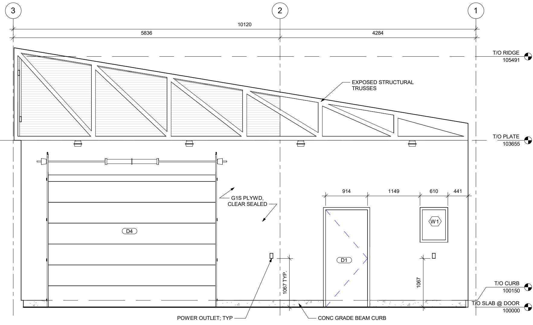
1 INT ELEVATION - GARAGE - C 1:50
