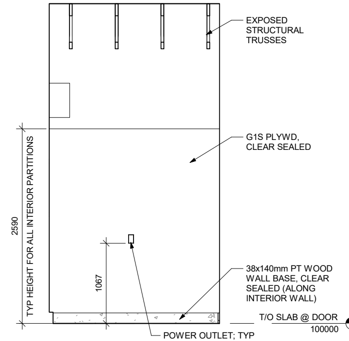
6 INT ELEVATION - STORAGE - B 1 : 50
