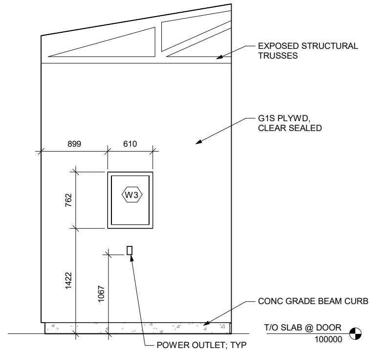
5 INT ELEVATION - STORAGE - A 1 : 50
