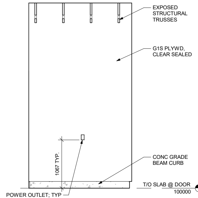
8 INT ELEVATION - STORAGE - D 1 : 50
