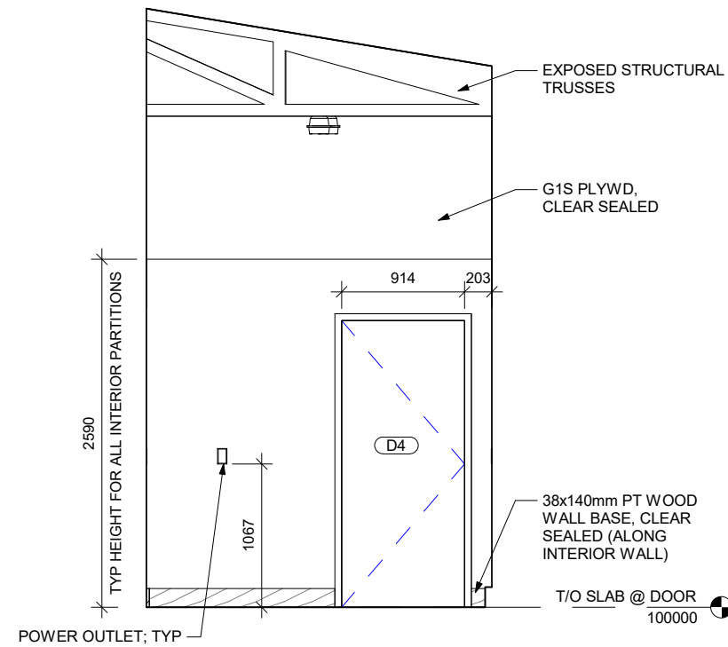
7 INT ELEVATION - STORAGE - C 1 : 50
