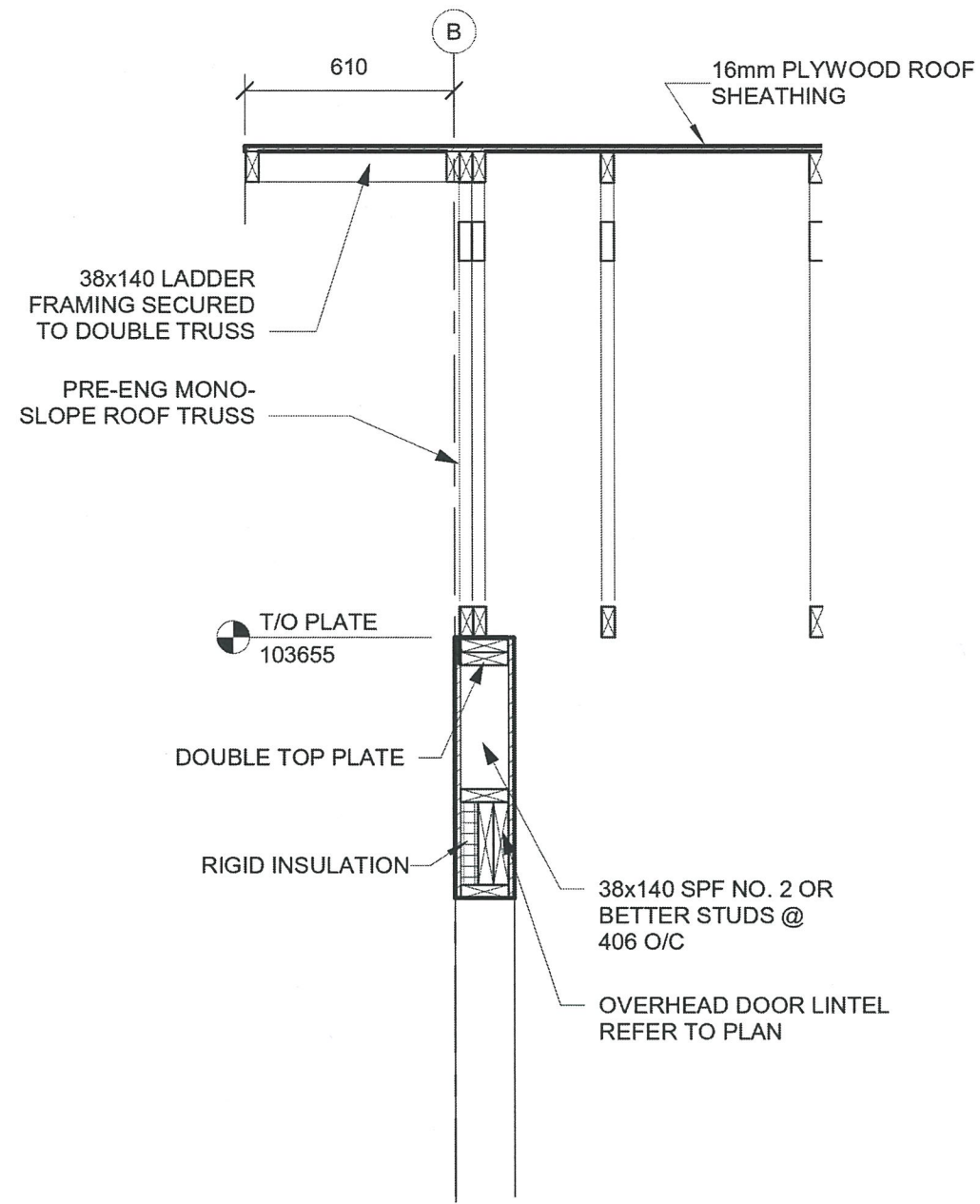
3 SECTION S502 1:20
