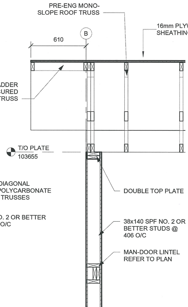
2 SECTION S502 1:20
