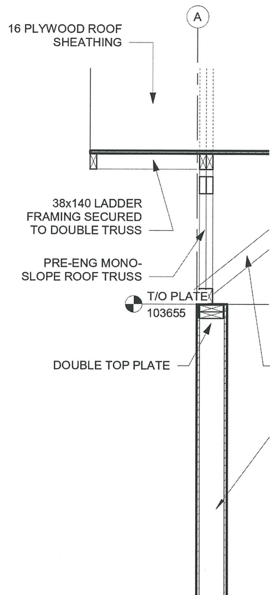
1 SECTION S502 1:20
