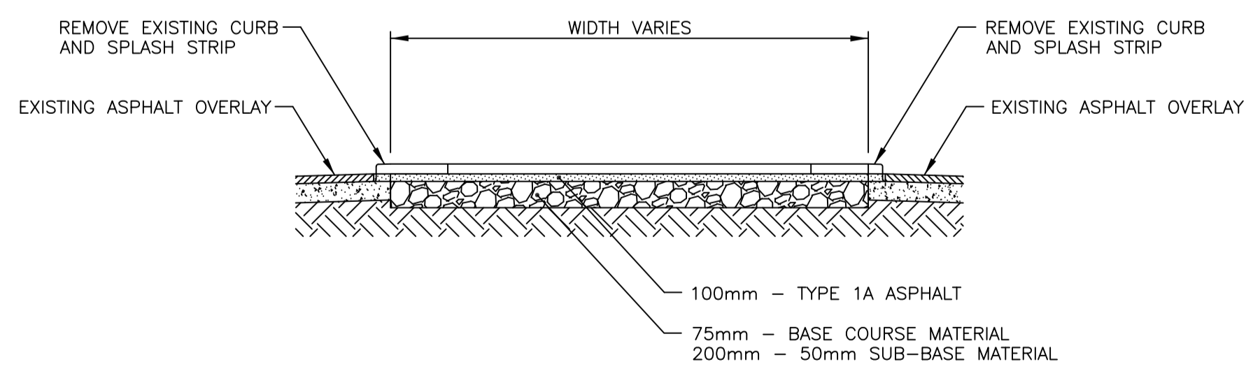
ASPHALT CROSS-OVER SECTION (TYPICAL) N.T.S.
