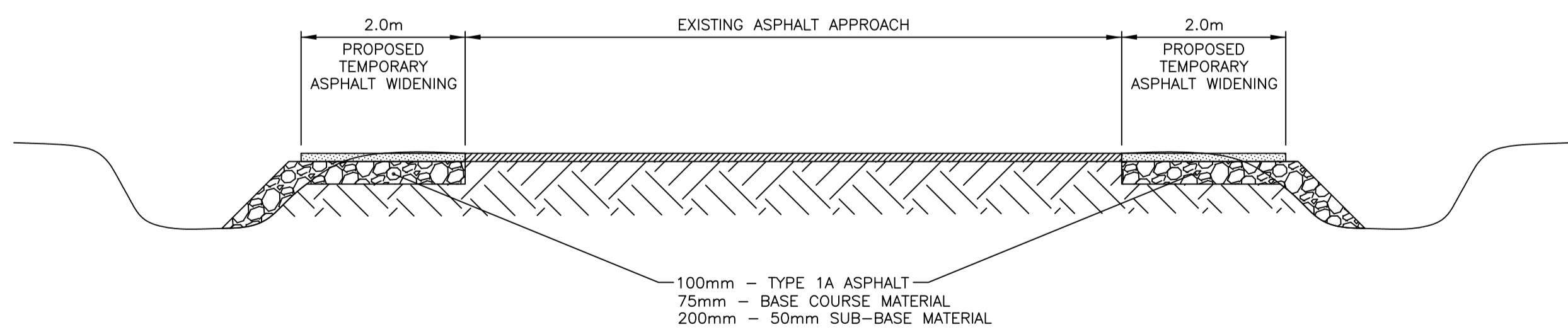
TEMPORARY ASPHALT APPROACH WIDENING (TYPICAL) N.T.S.
