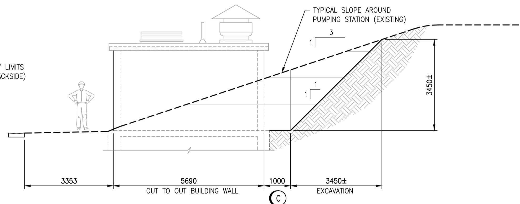
NORTH ELEVATION 1 : 75
