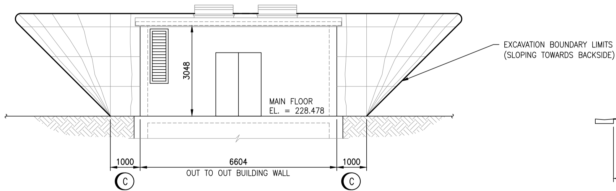
EAST ELEVATION 1 : 75
