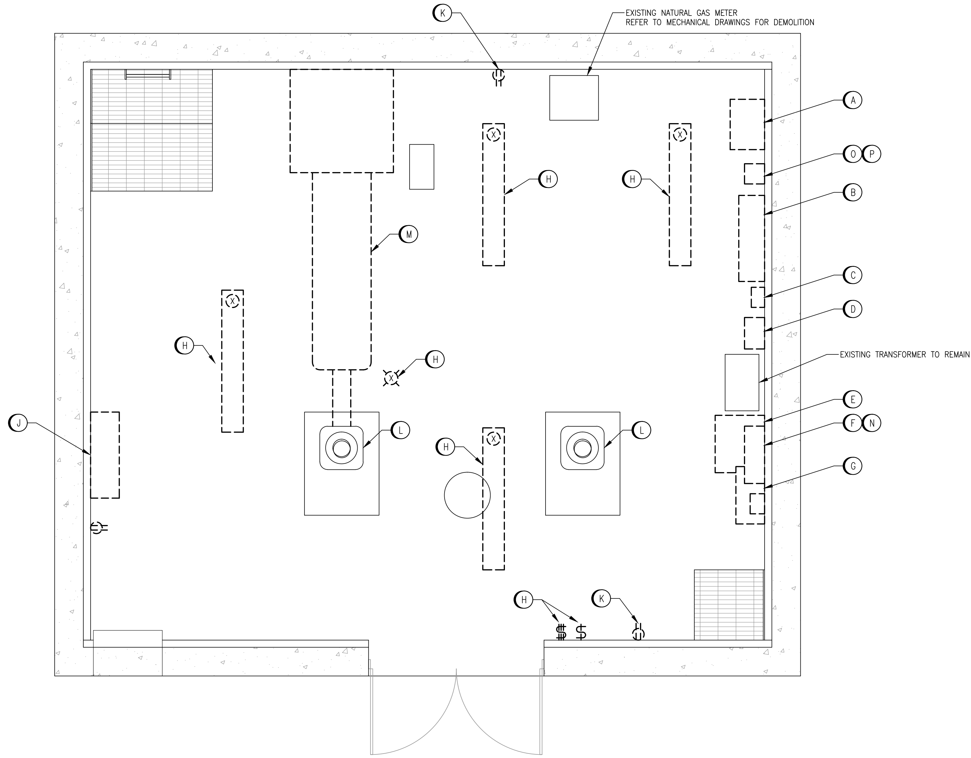
MAIN FLOOR PLAN SCALE: 1 : 20
