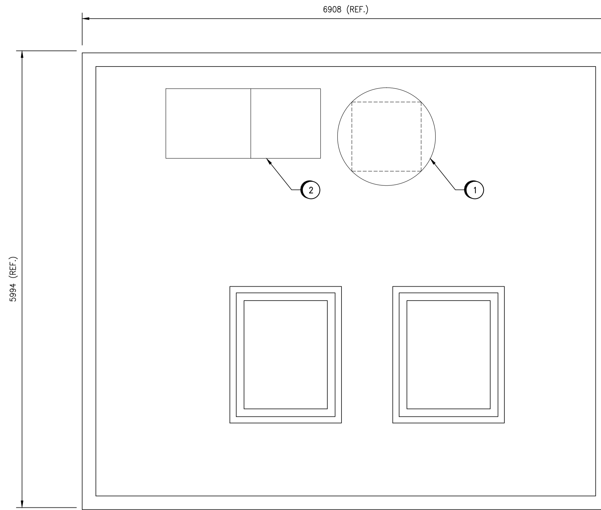
ROOF PLAN - REMOVALS SCALE: 1 : 30
