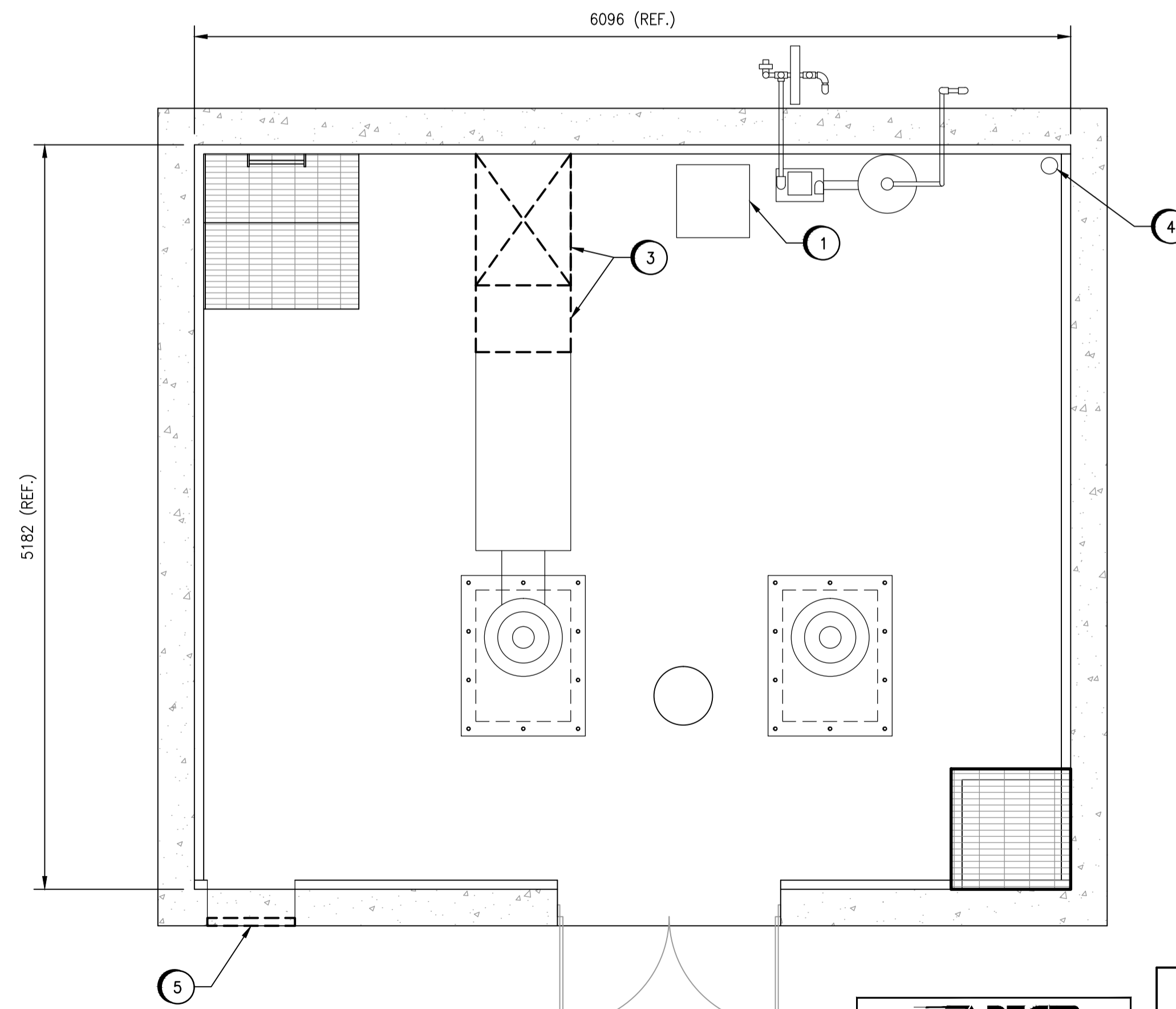
MAIN FLOOR PLAN - REMOVALS SCALE: 1 : 30
