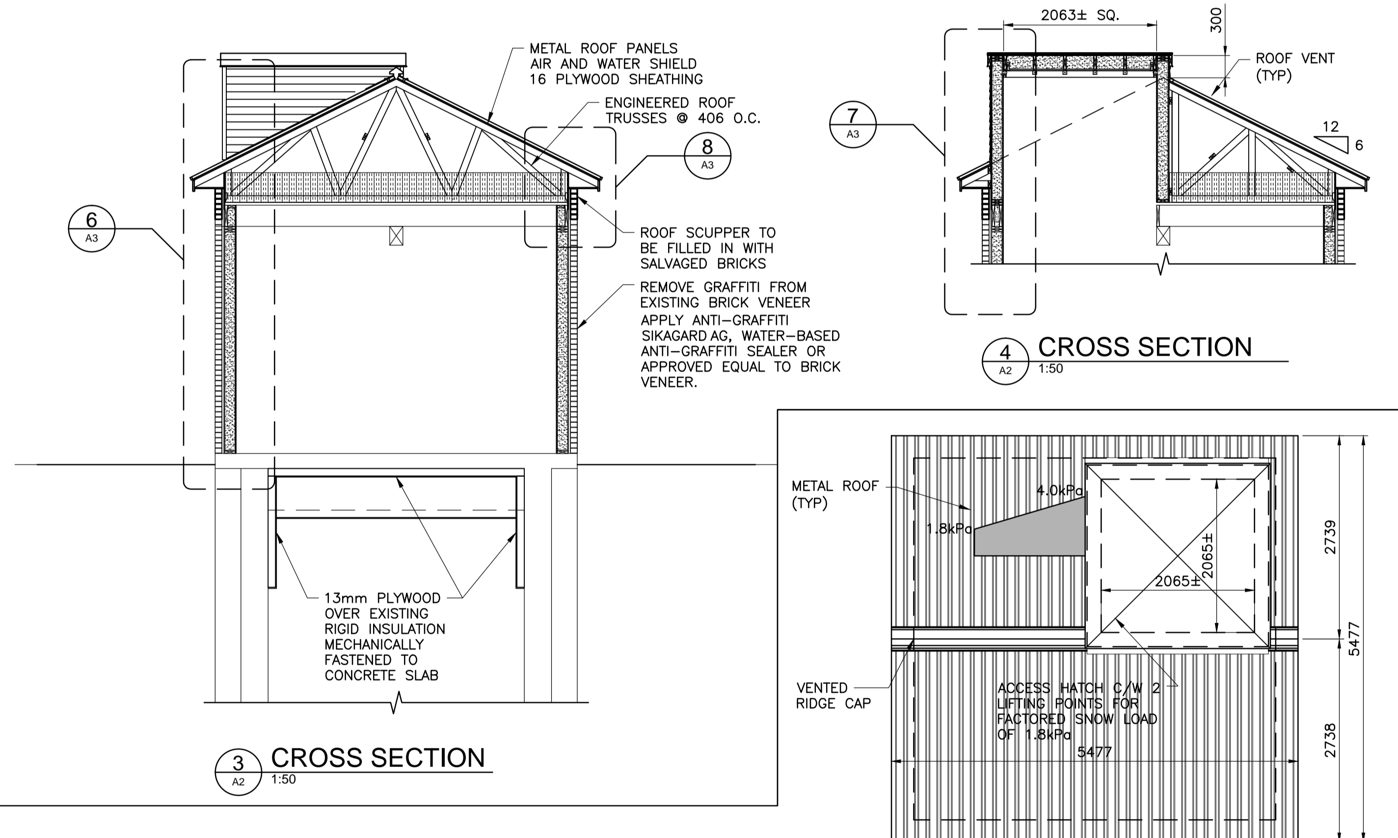
ROOF PLAN WITH SNOW LOADINGS 1:50
