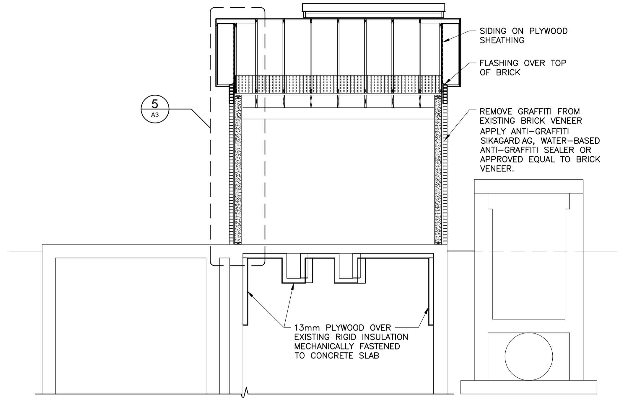
2 CROSS SECTION 1:50
