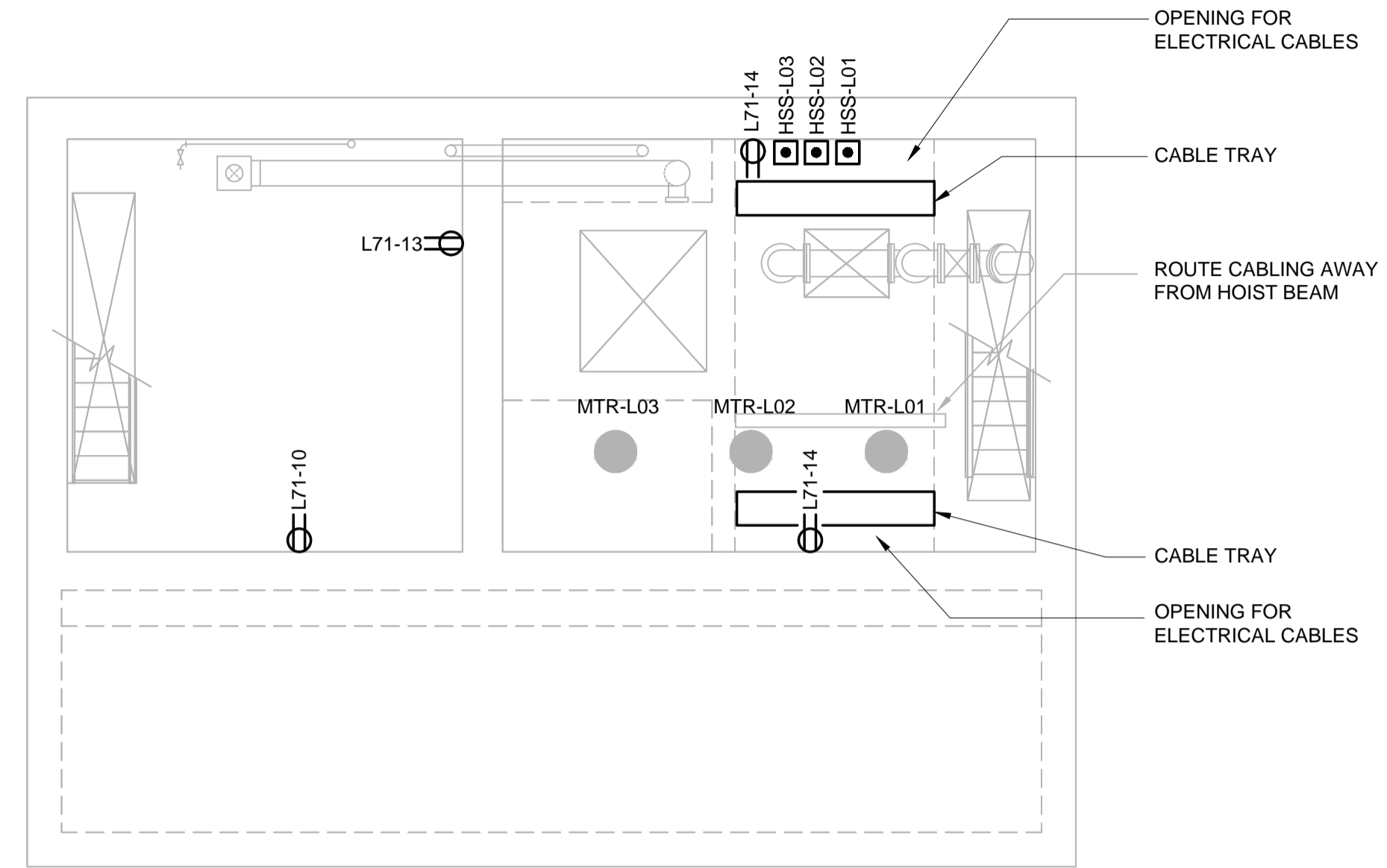
COMM. ROOM, PUMP MOTOR ROOM FLOOR PLAN 1:50
