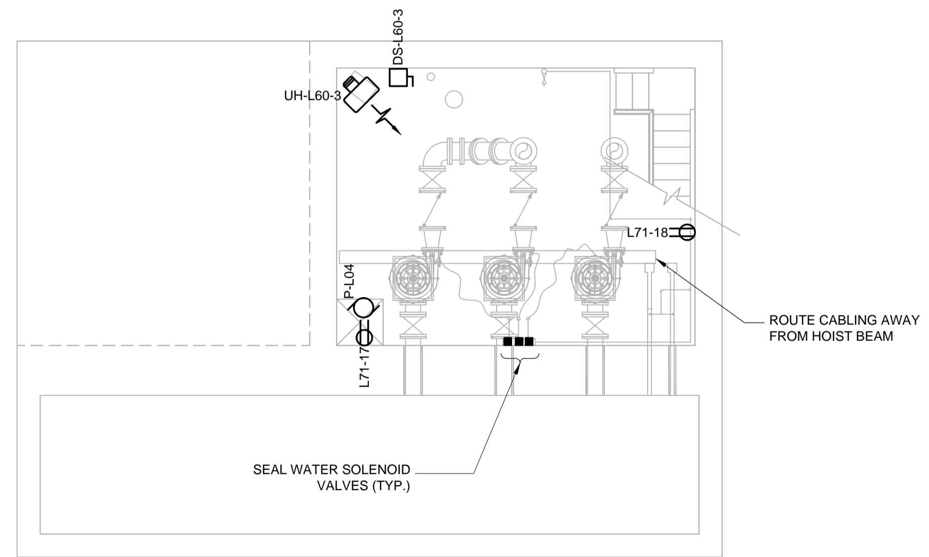
PUMP ROOM FLOOR PLAN 1:50
