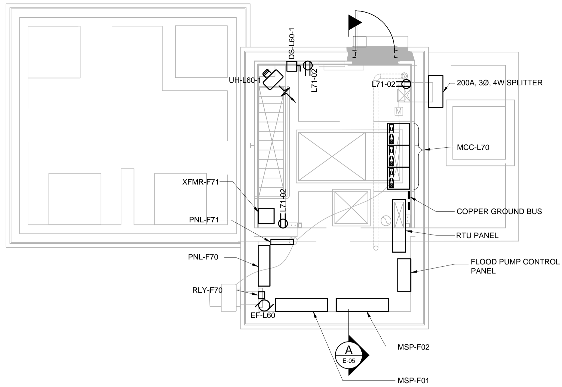
ENTRY LEVEL FLOOR PLAN 1:50
