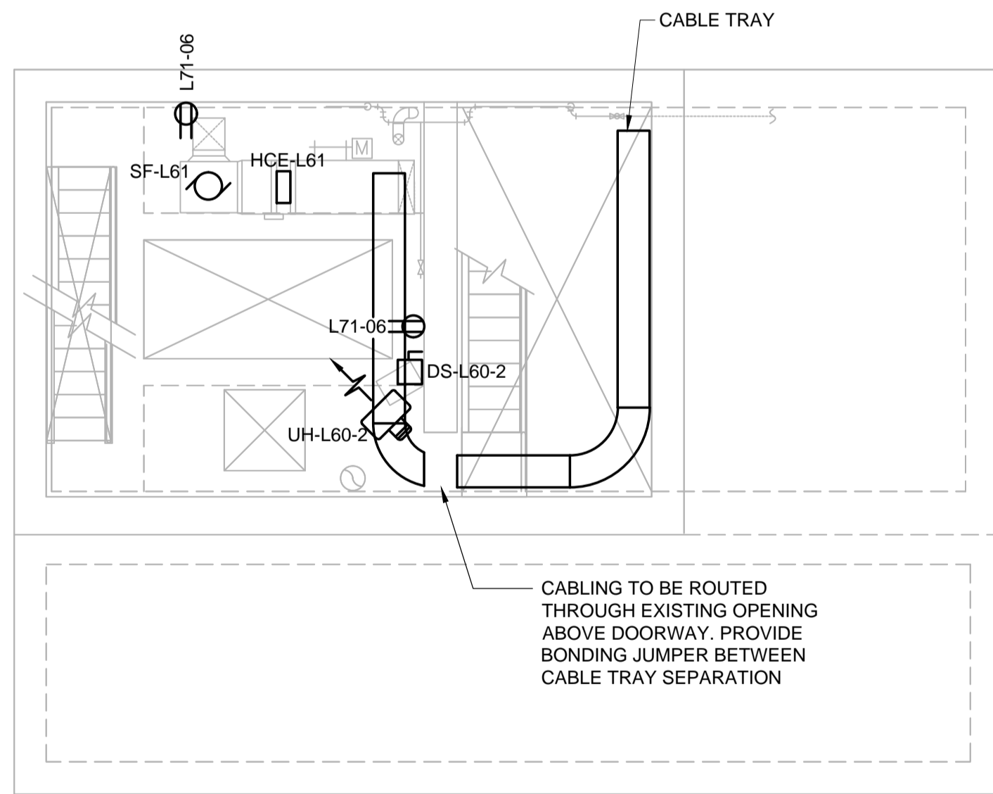
COMM. MOTOR ROOM FLOOR PLAN 1:50
