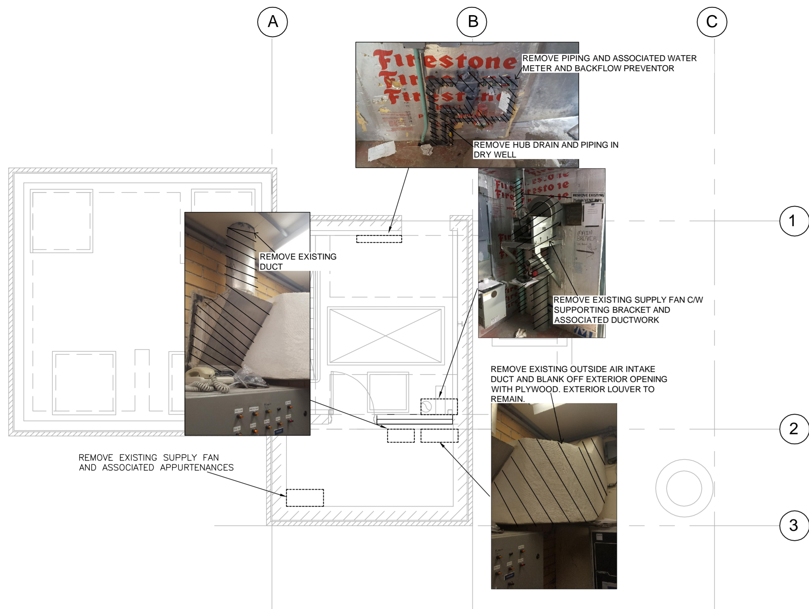
DEMOLITION ENTRY LEVEL FLOOR PLAN 1:50
