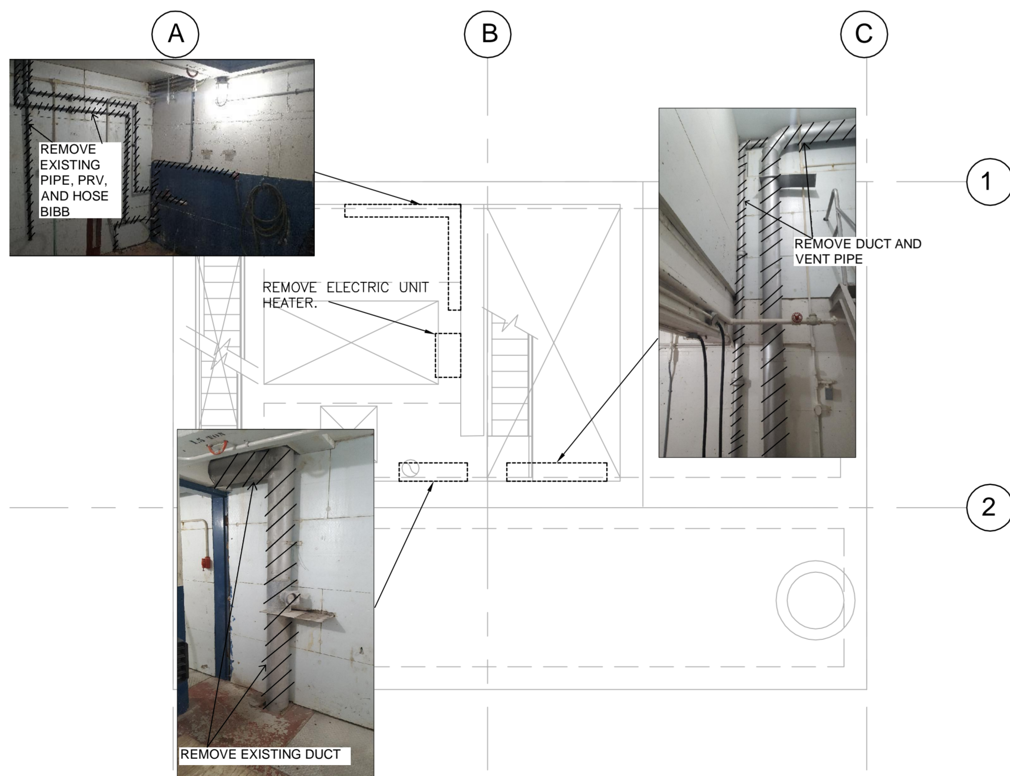
DEMOLITION COMM & MOTOR ROOM FLOOR PLAN 1:50
