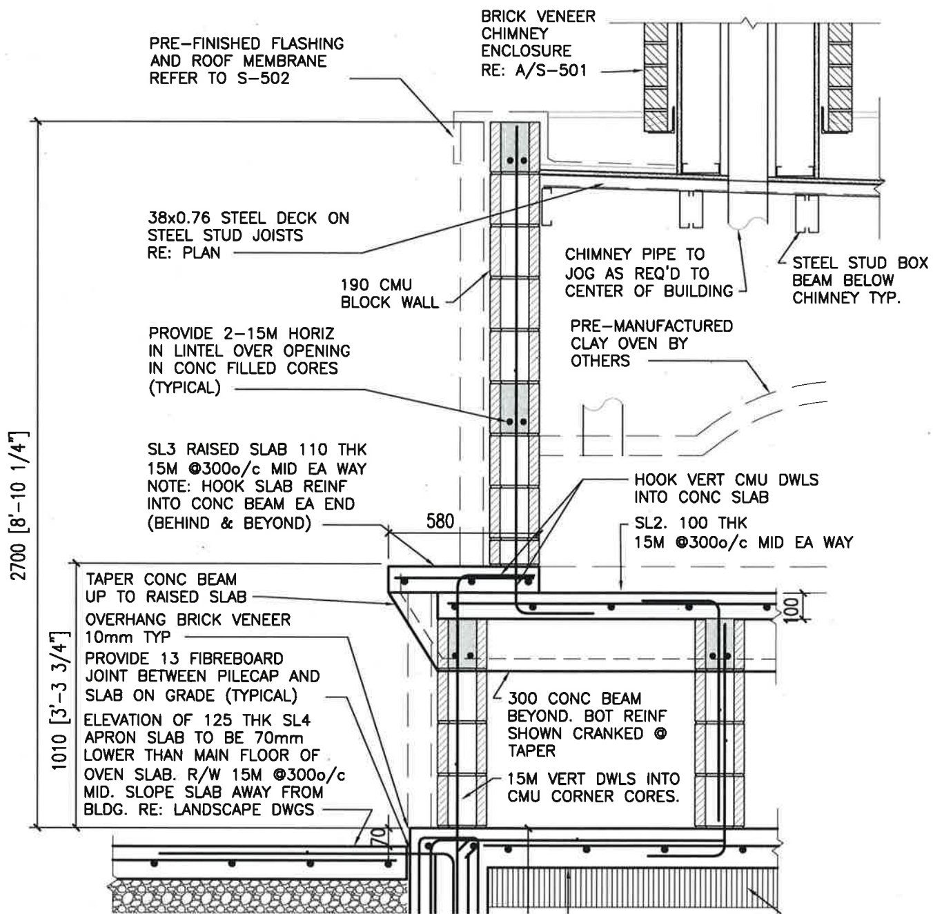
B WALL SECTION S-301 1:20
