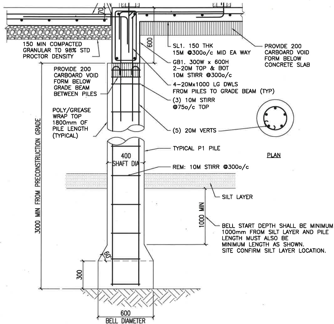
A TYPICAL P1 PILE S-301 1:20
