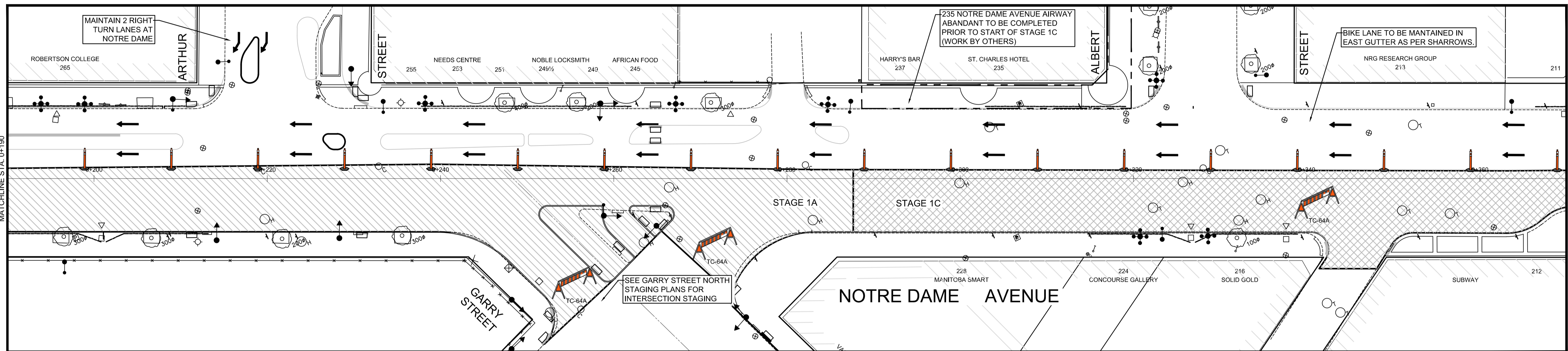
PLAN - STAGE 1 Scale 1:250
