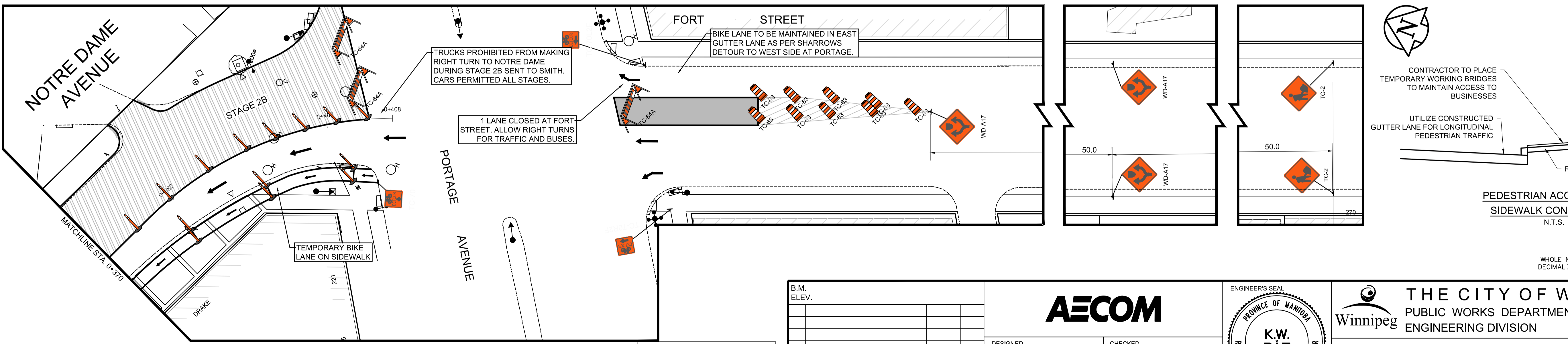
PLAN - STAGE 2 Scale 1:250
