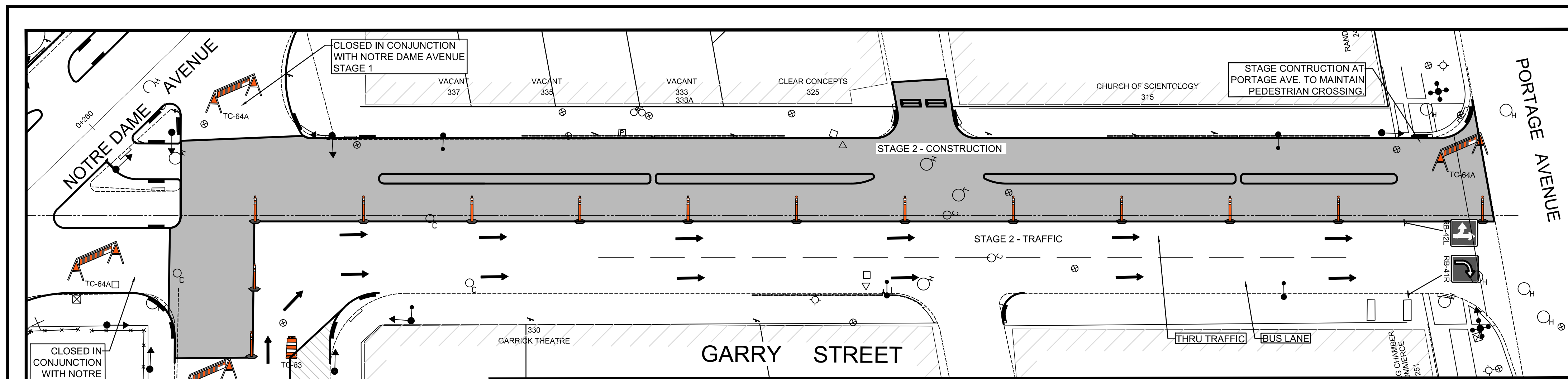
PLAN - STAGE 2 Scale 1:250
