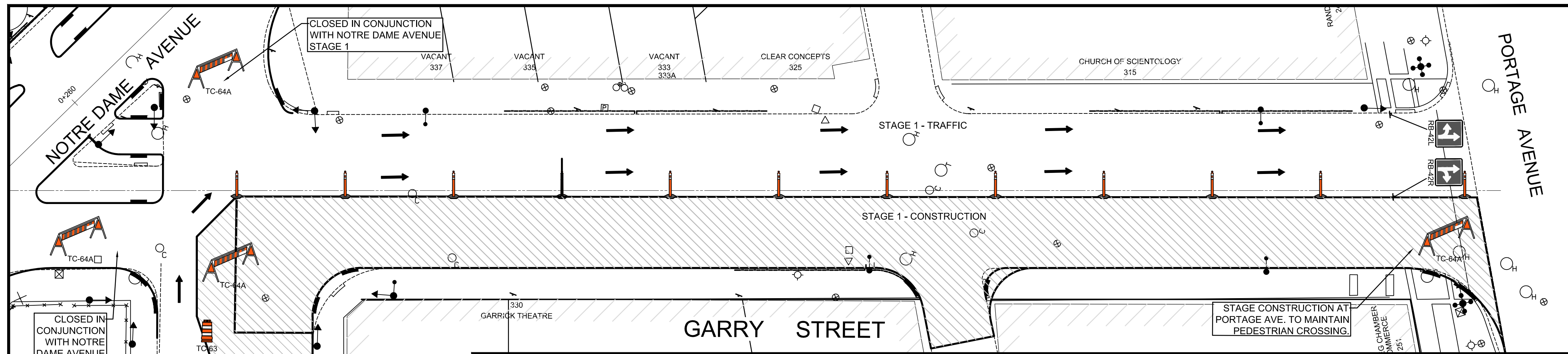
PLAN - STAGE 1 Scale 1:250
