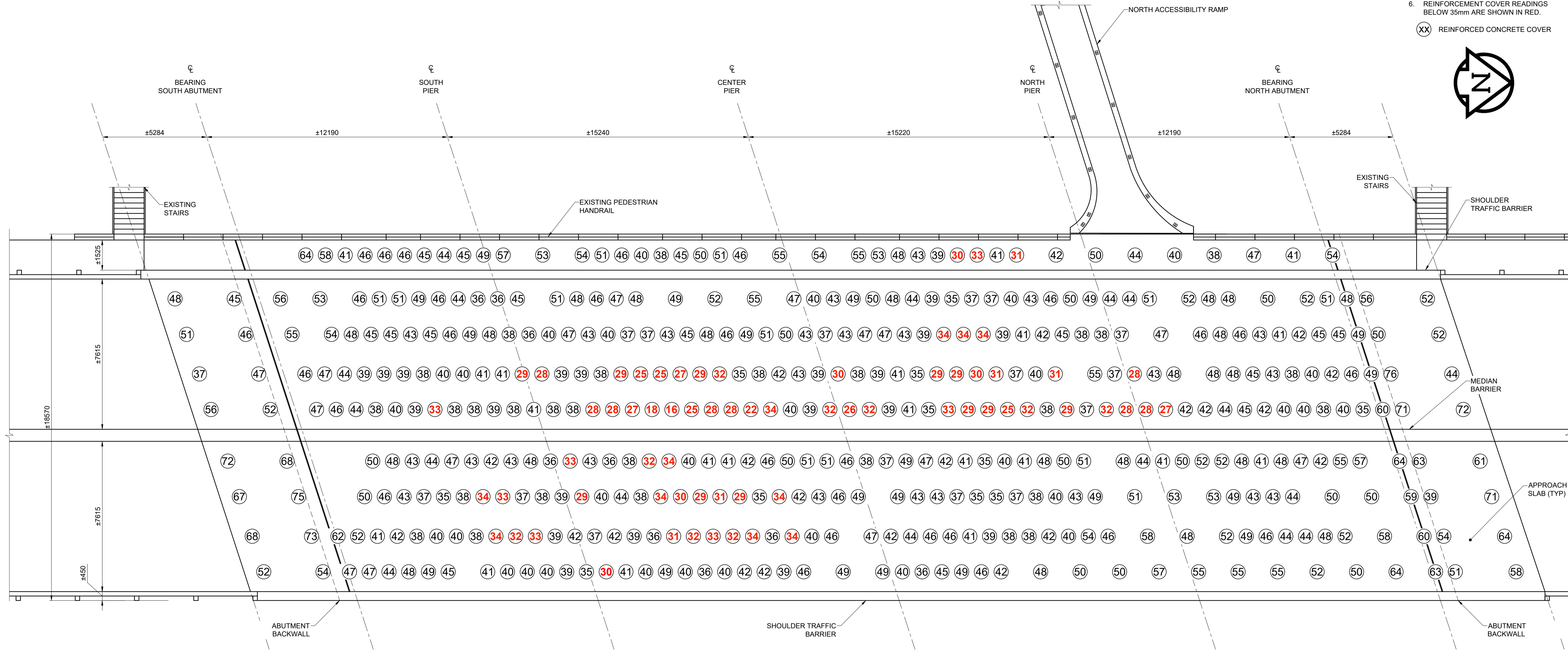
PLAN OF REBAR COVER READINGS ON EXISTING DECK AND APPROACH SLABS SCALE 1:100
