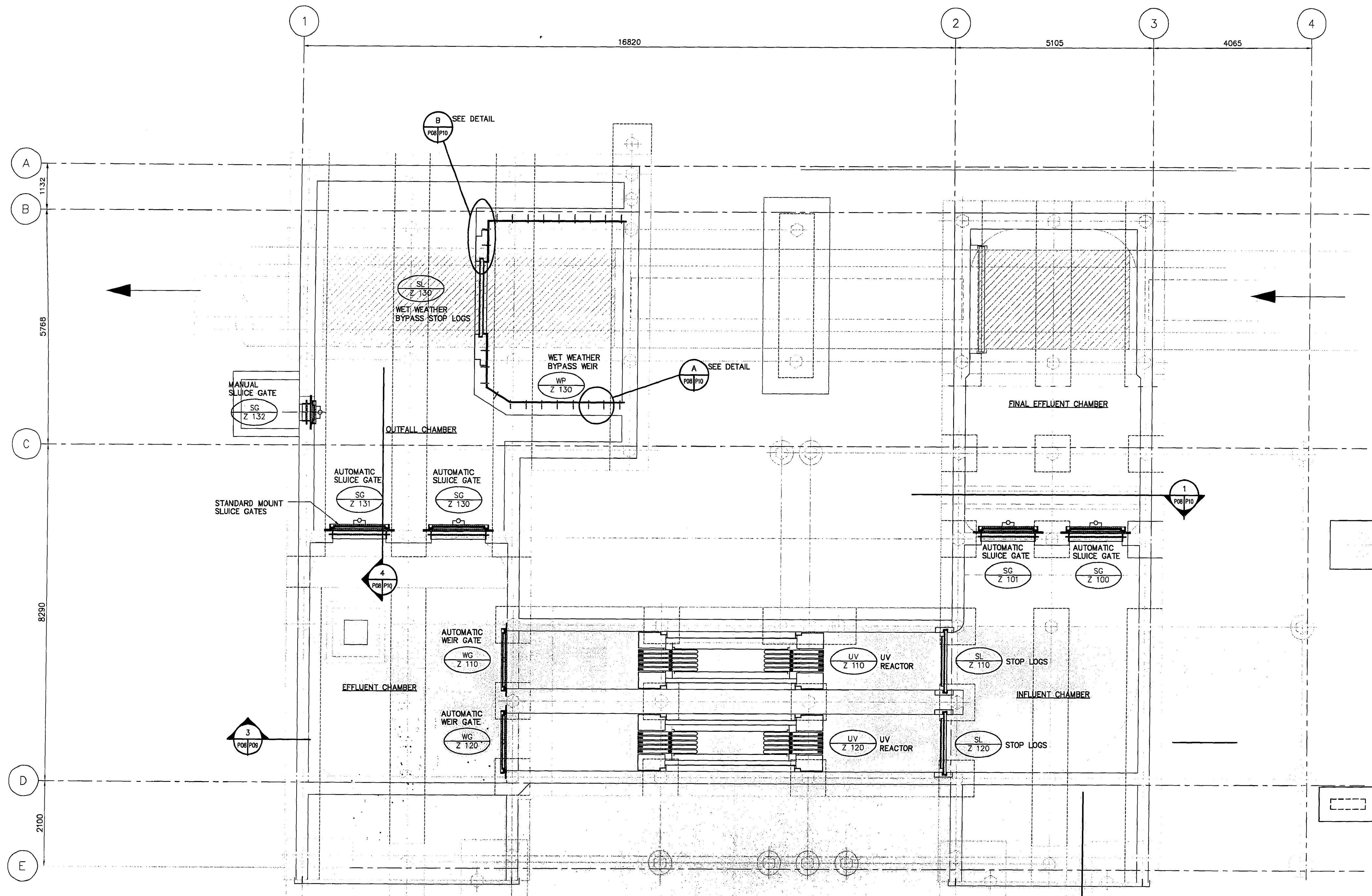
LOWER FLOOR PLAN SCALE 1:50
