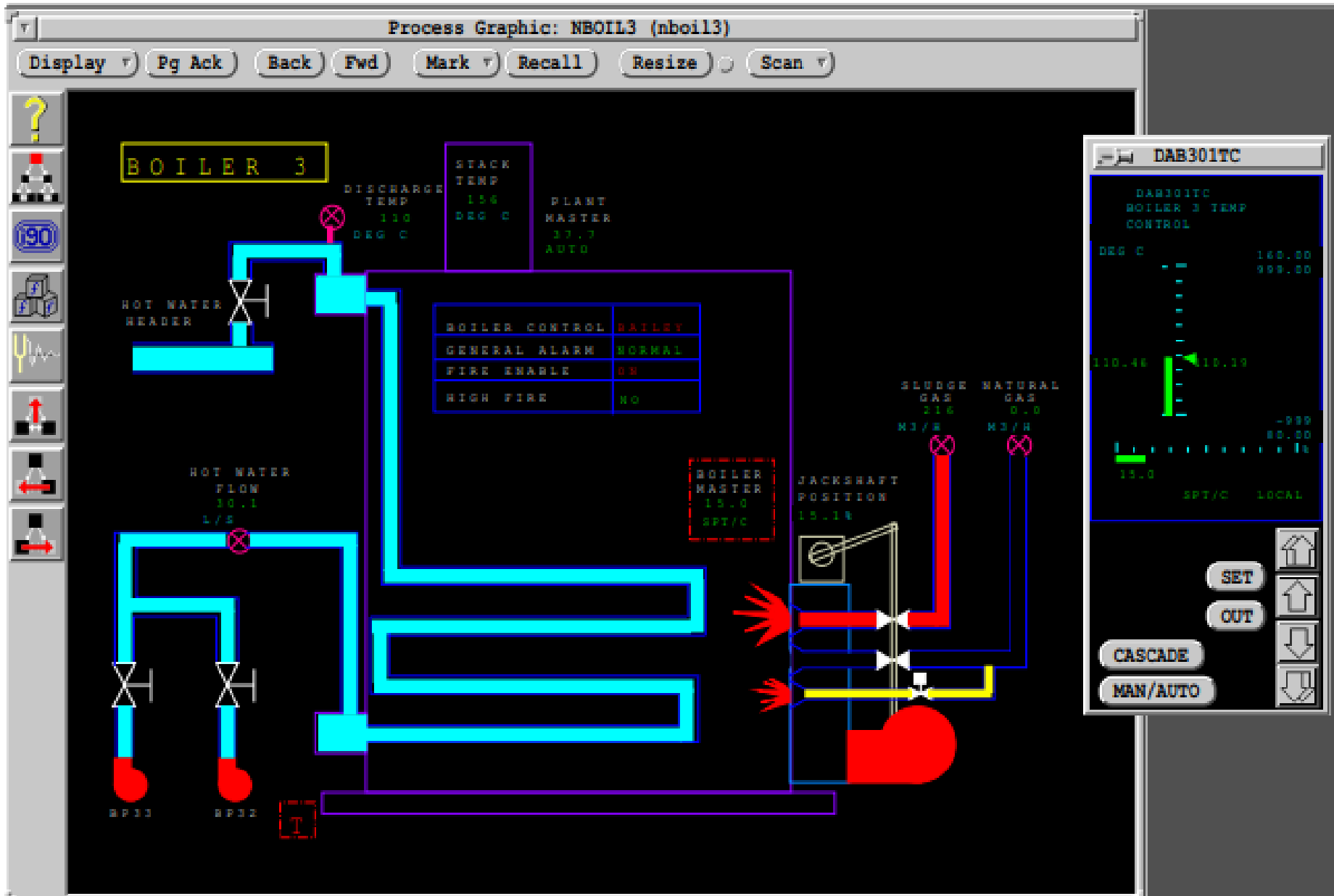
Figure 4: Boiler 3 DCS Screenshot
