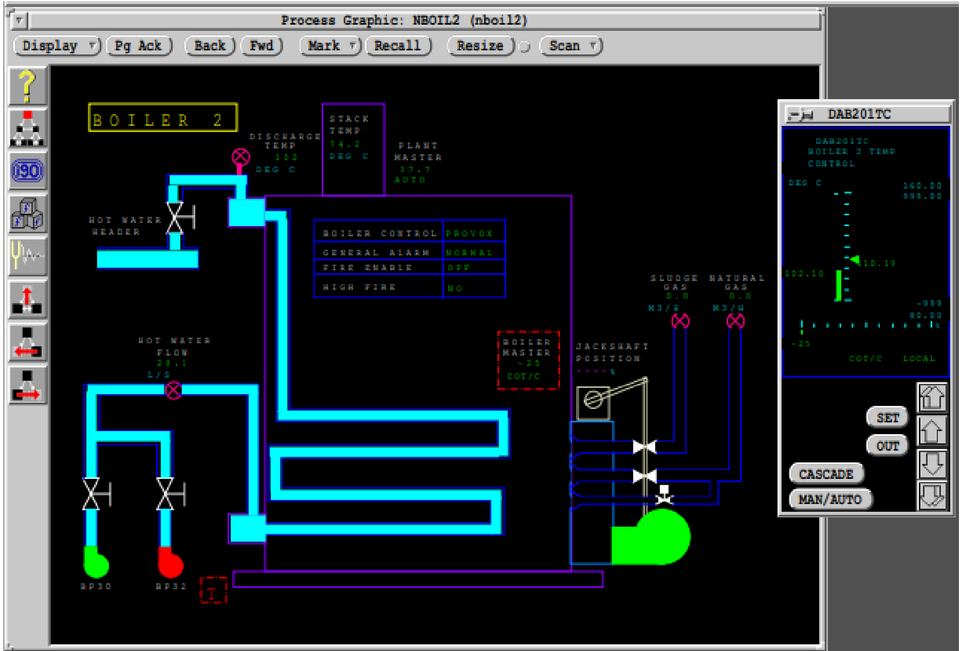
Figure 3: Boiler 2 DCS Screenshot
