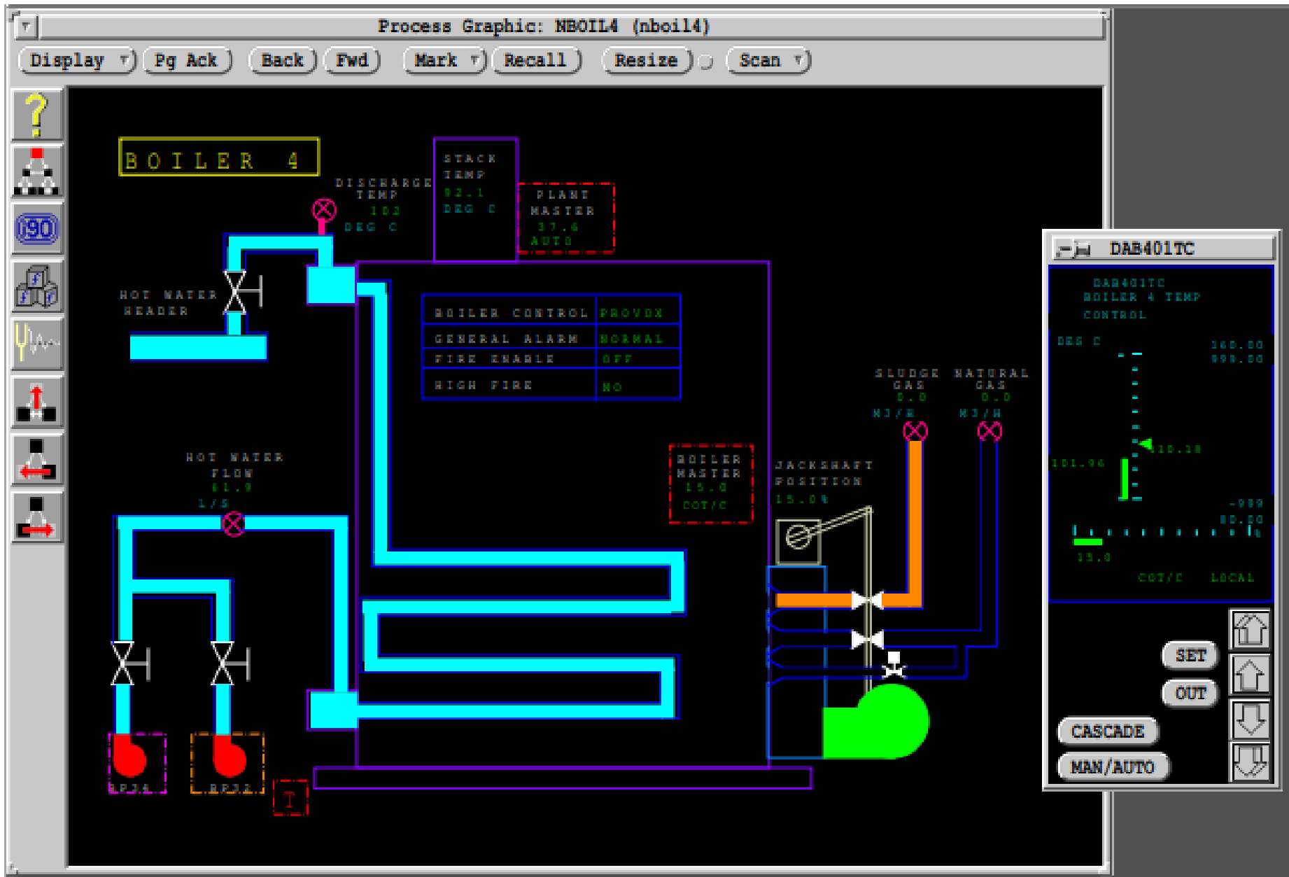
Figure 5: Boiler 4 DCS Screenshot
