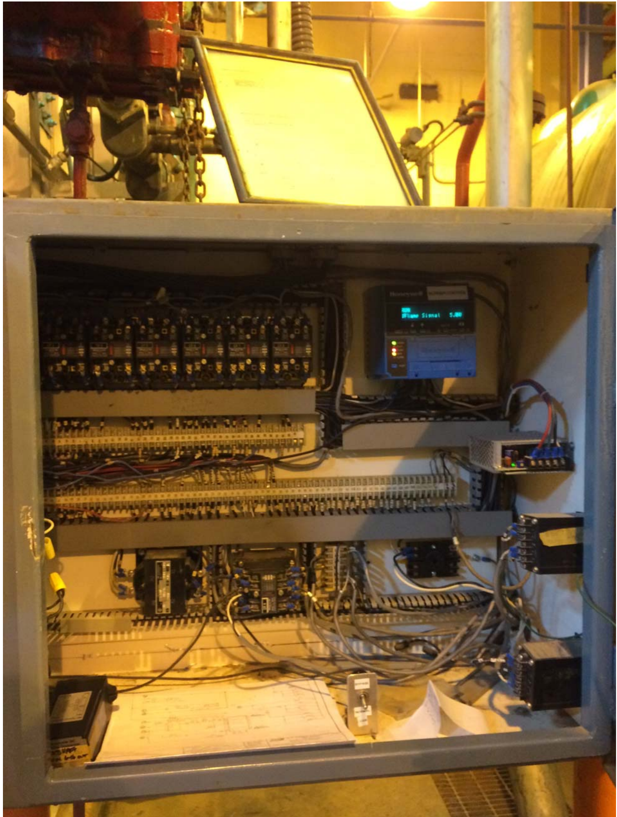
Figure 2: Partial interior view of a local control panel (Typical of Boilers 1, 2 &3)
