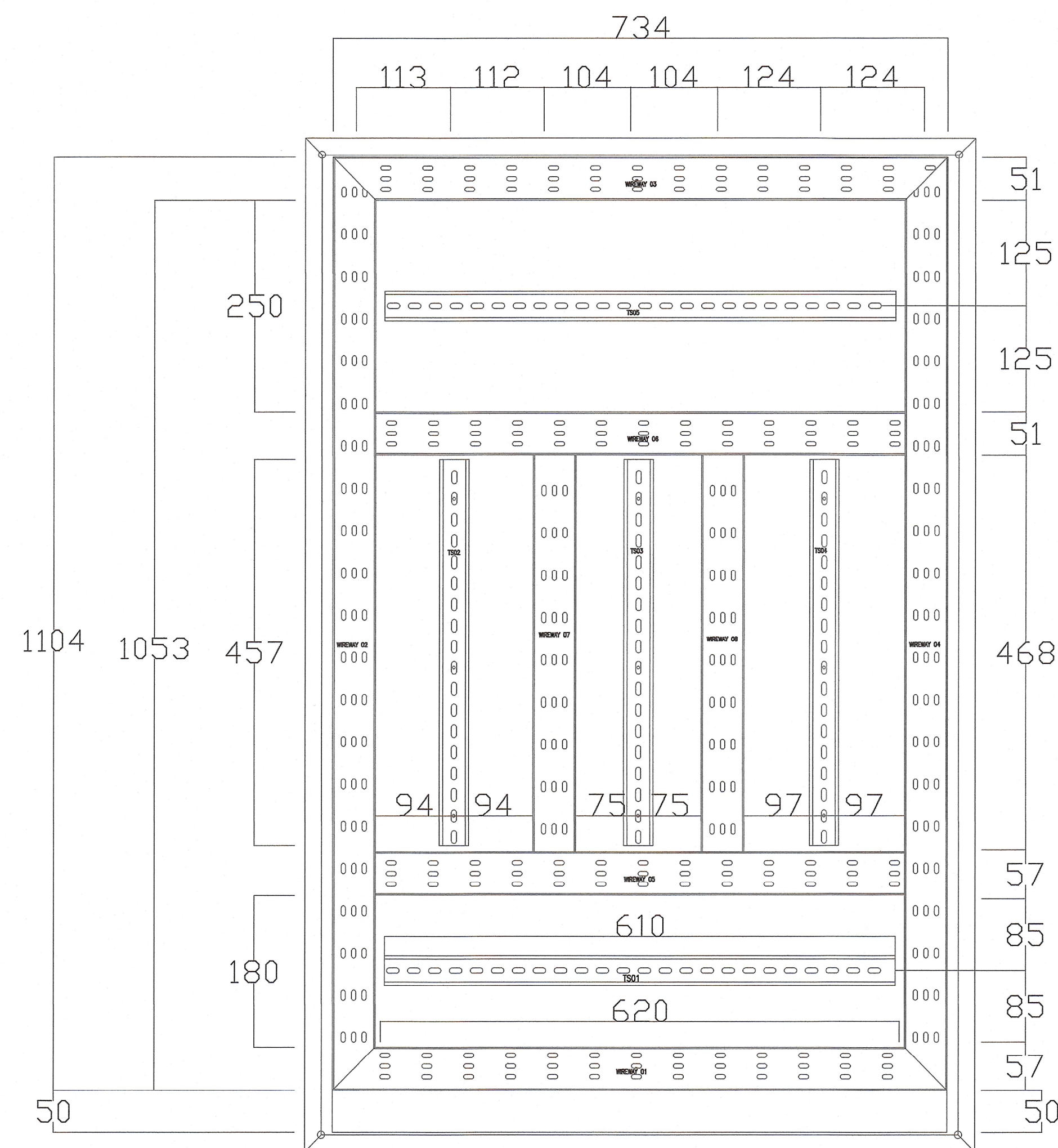
RTU BACK PLATE CUT-OUT BACK PLATE
