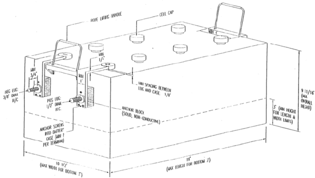
BUS BATTERY WITH DROP TERMINALS - Dimensional Specifications -
