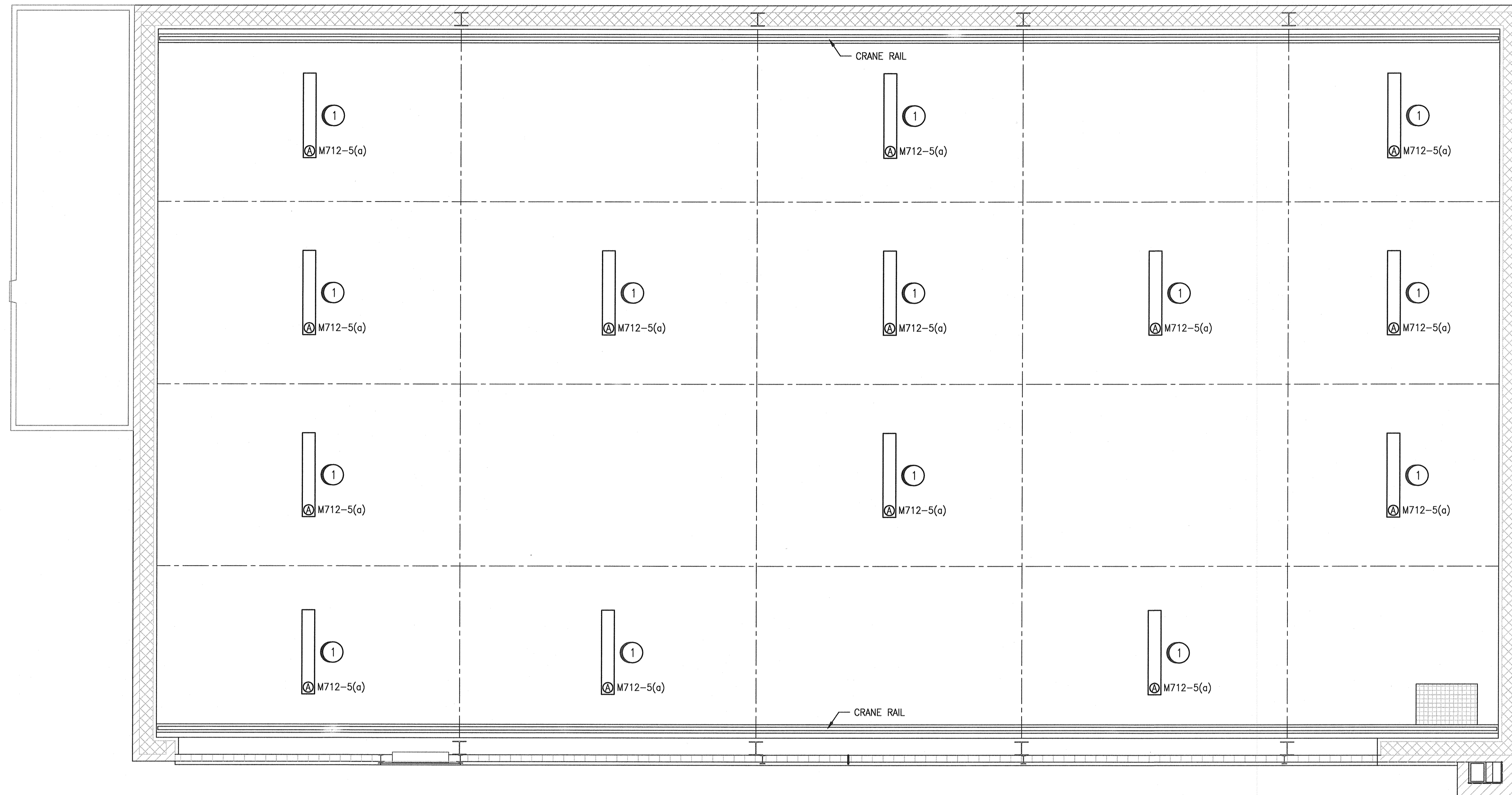
MAIN FLOOR PLAN SCALE: 1 : 40
