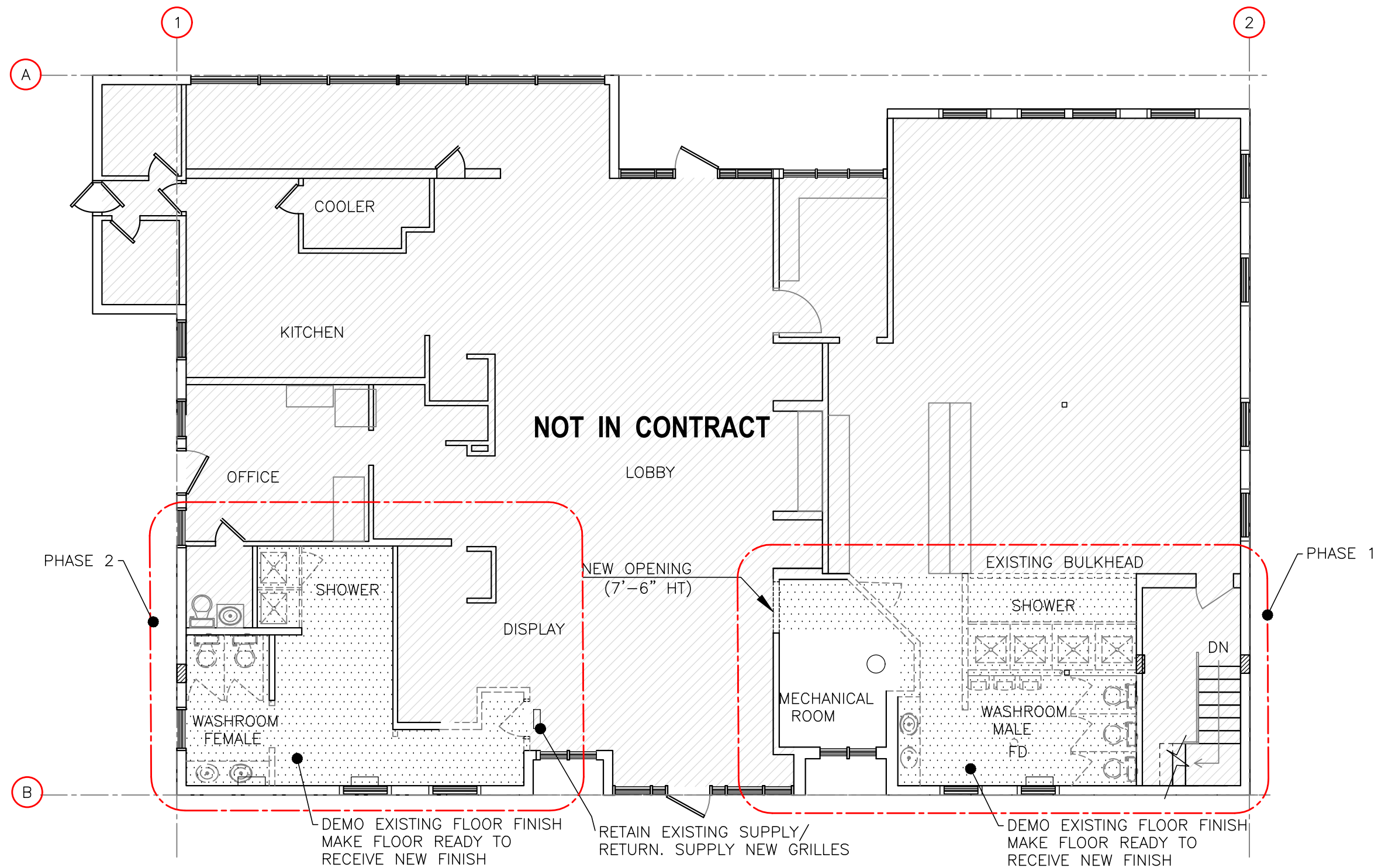
DEMOLITION PLAN SCALE: 1/8"=1'-0"
