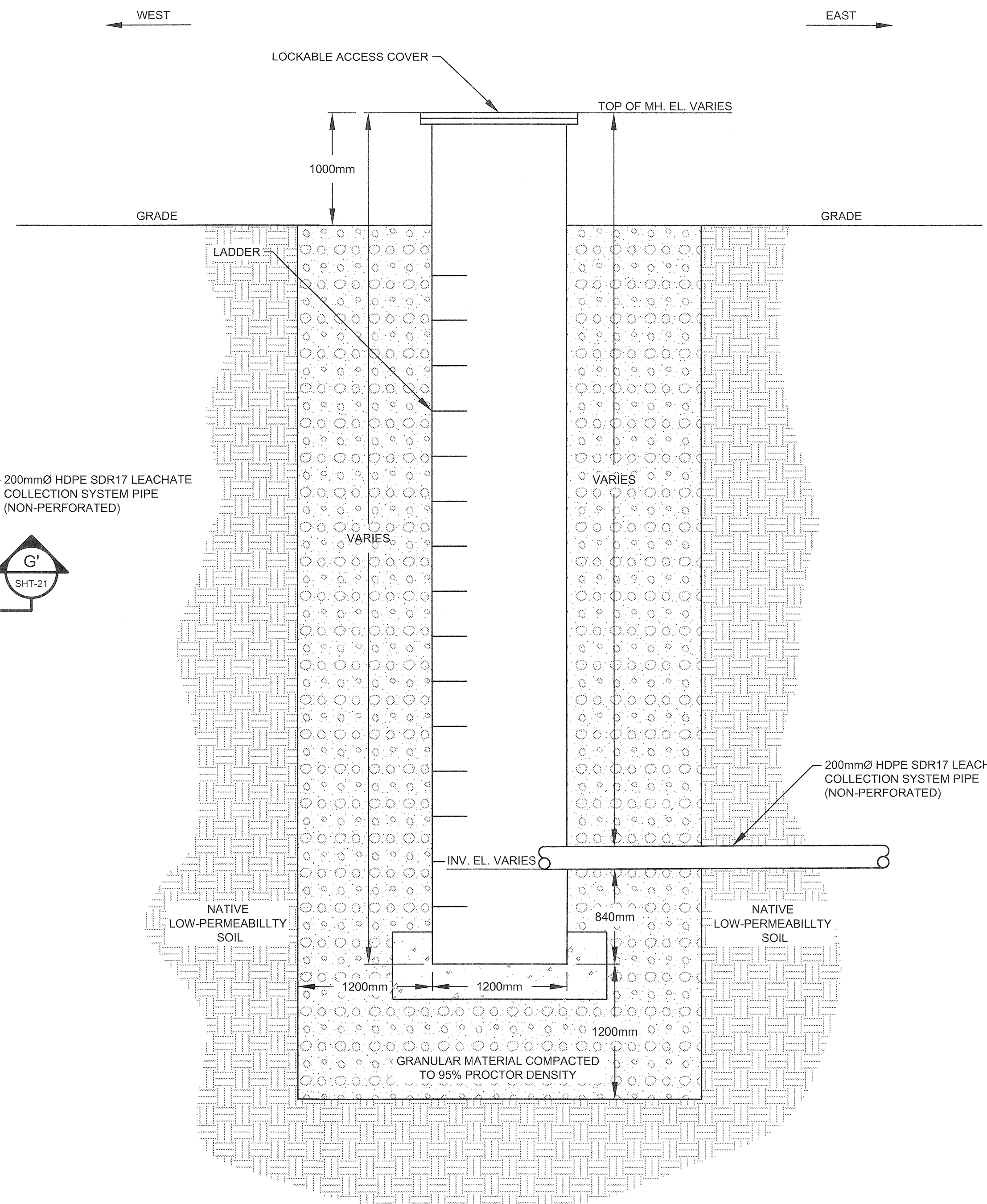
SECTION G-G'
