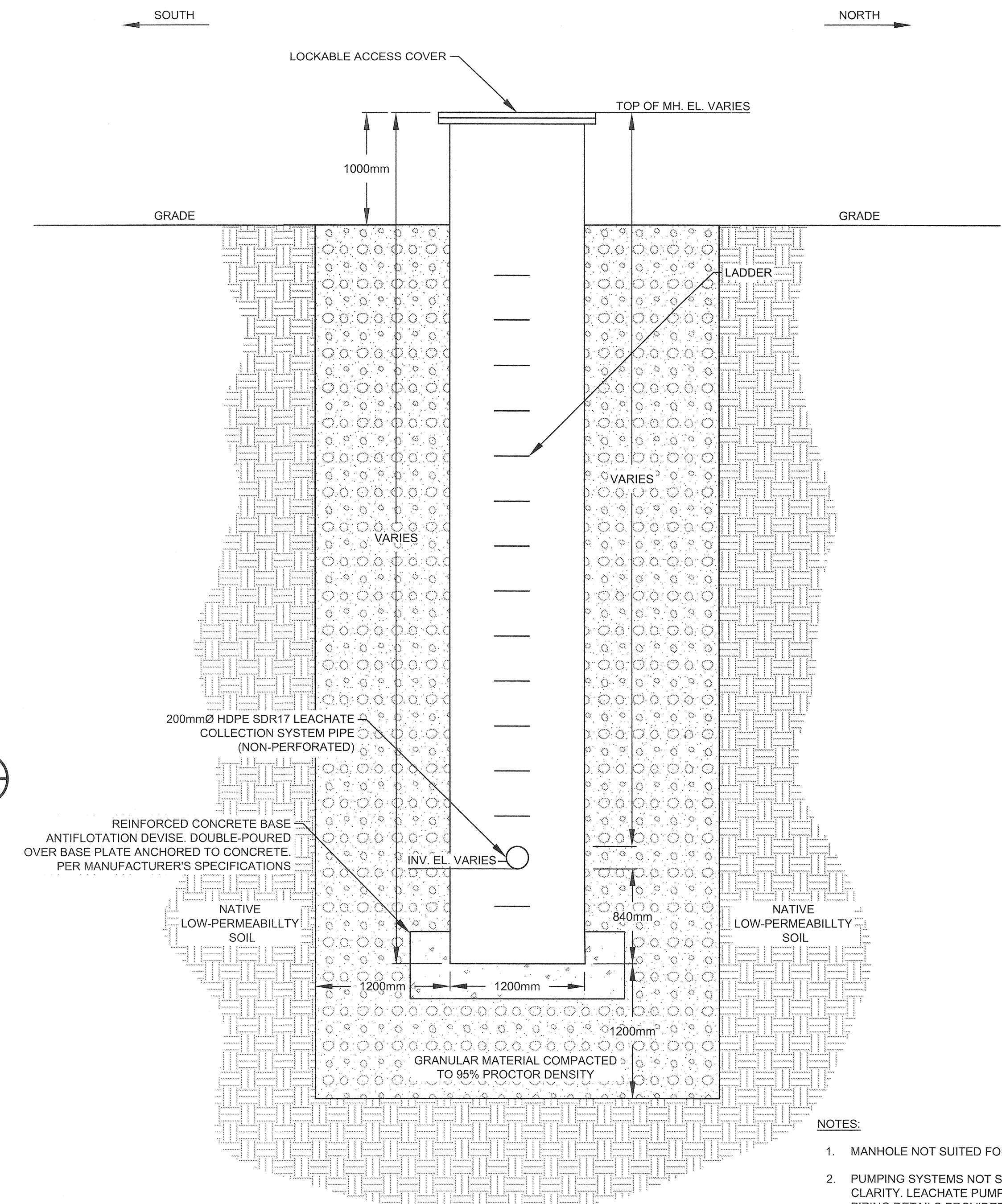
SECTION H-H'
