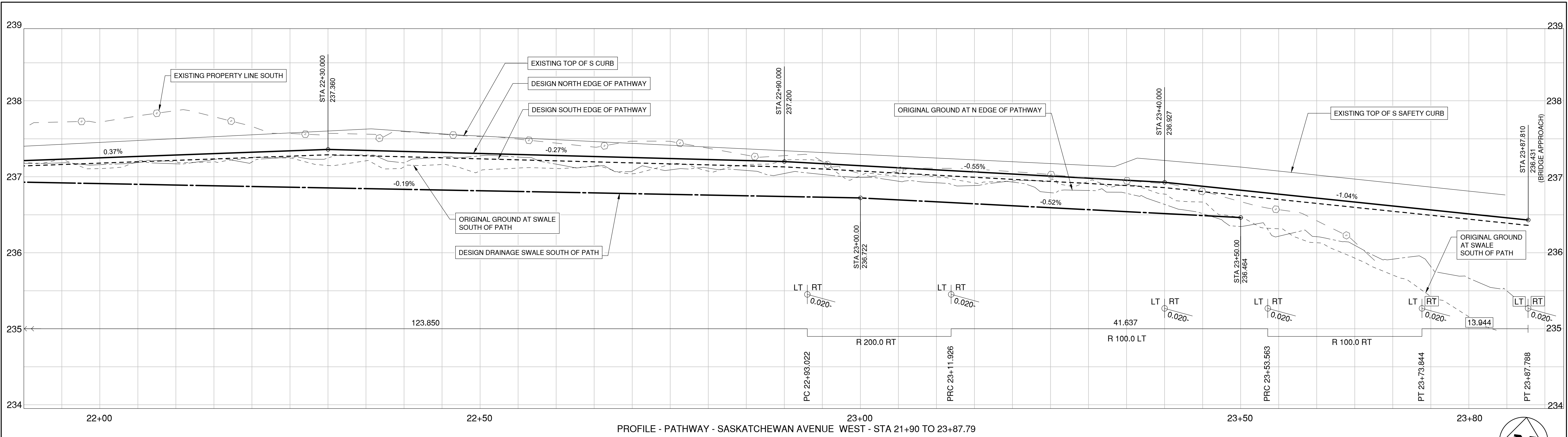
PROFILE - PATHWAY - SASKATCHEWAN AVENUE WEST - STA 21+90 TO 23+87.79
