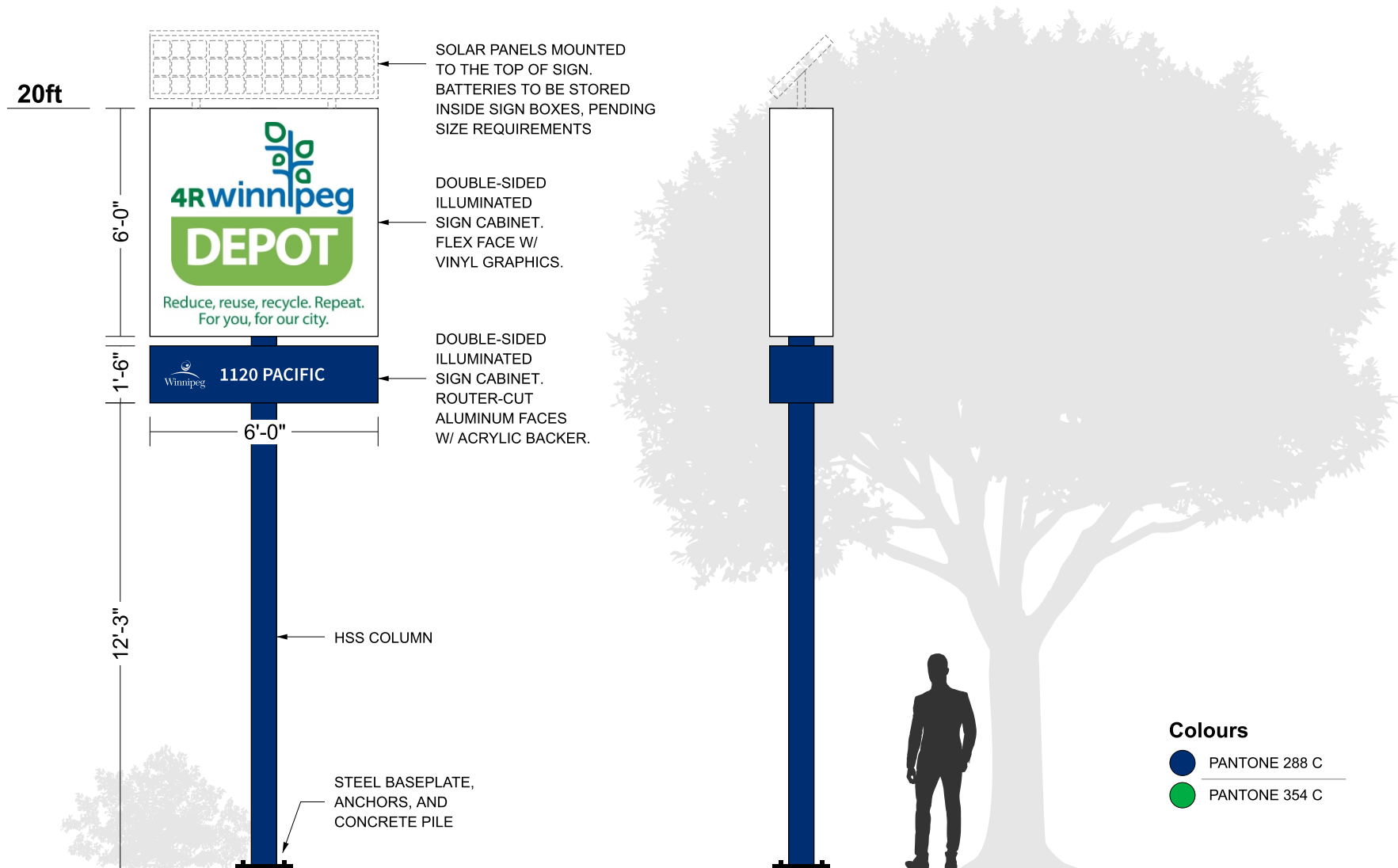
1 Single Pole Pylon Sign SCALE 1:24
